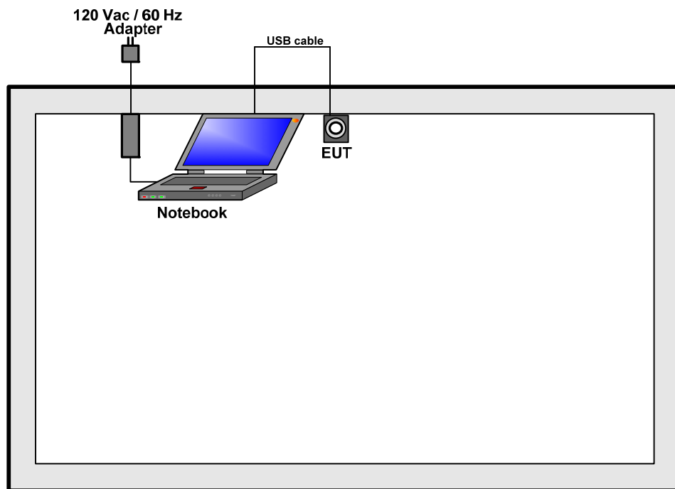
Test Setup Diagram - Radiated Mode 1 (Below 1GHz)
