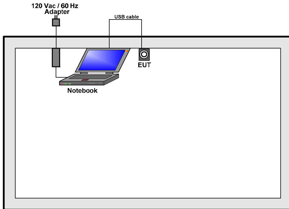
Test Setup Diagram - Radiated Emission Test Mode 1 (Below 1GHz)
