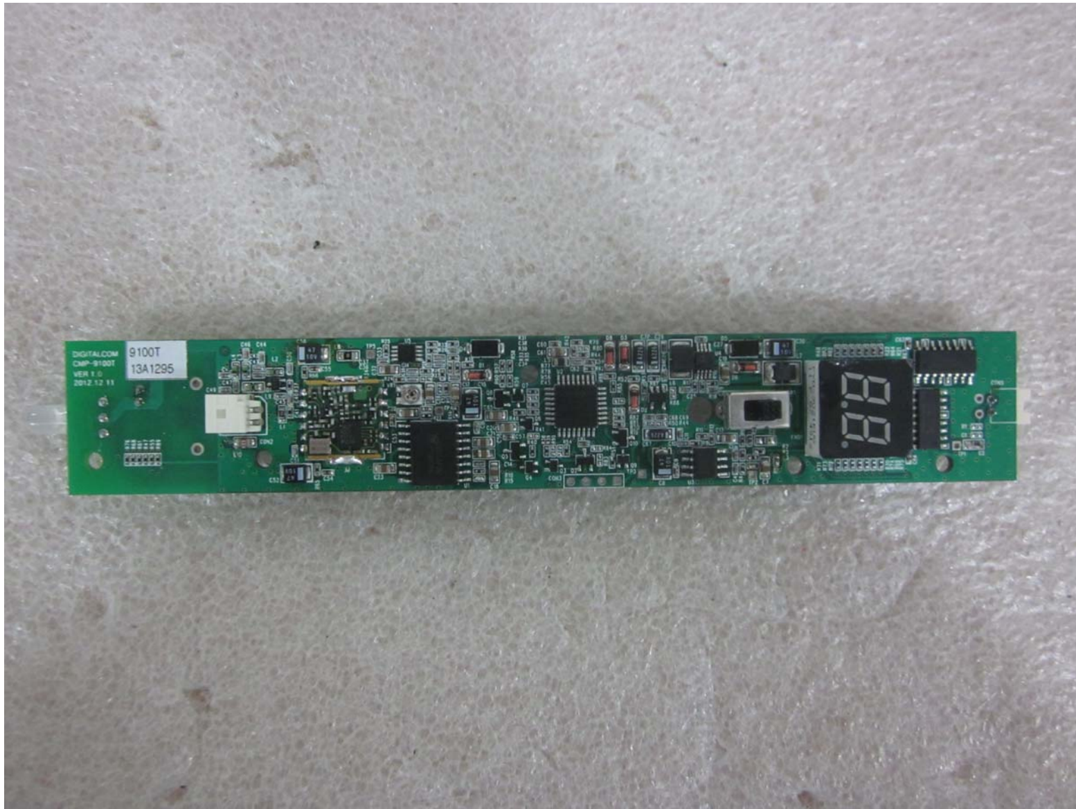
CMP-9100TF_Front of Main Board
