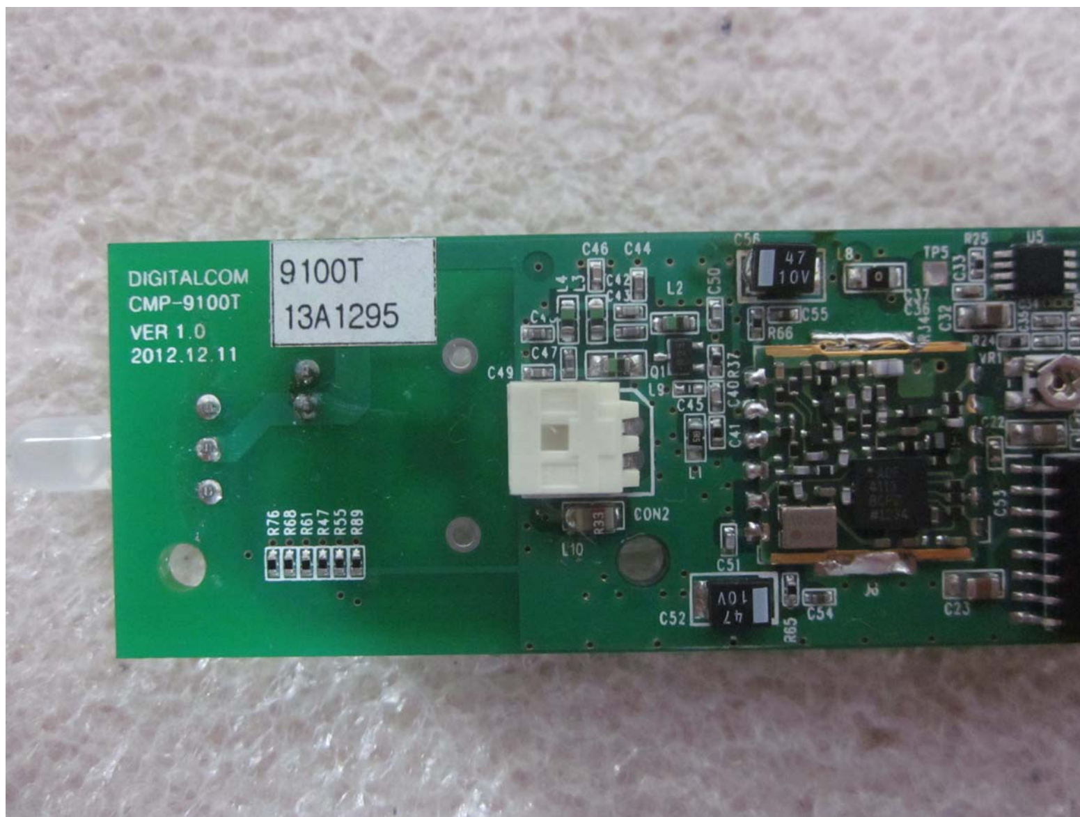
CMP-9100TF_Front of Main Board-1
