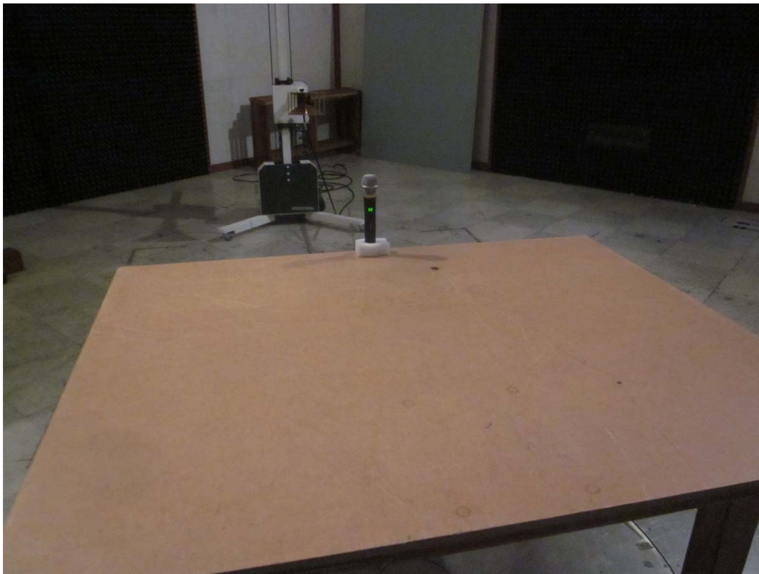
Radiated Emission_Above 1 GHz_Front
