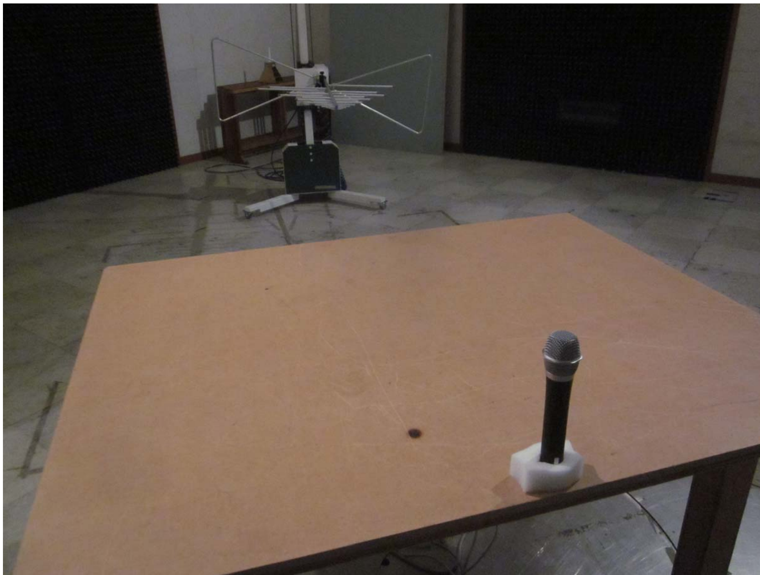
Radiated Emission_Below 1 GHz_Rear
