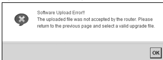
Figure 86 Error Message
