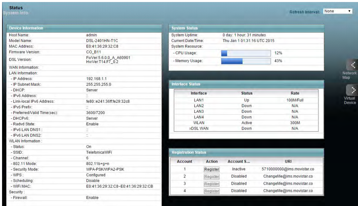
Figure 7 System Info
