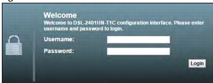
Figure 2-1 Password Screen
