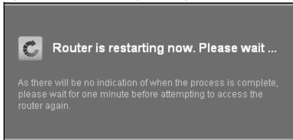
Figure 84 Firmware Uploading
