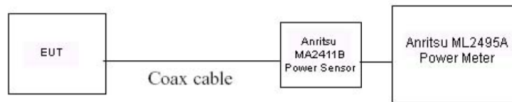
Figure 8-3 Power Measurement Setup
