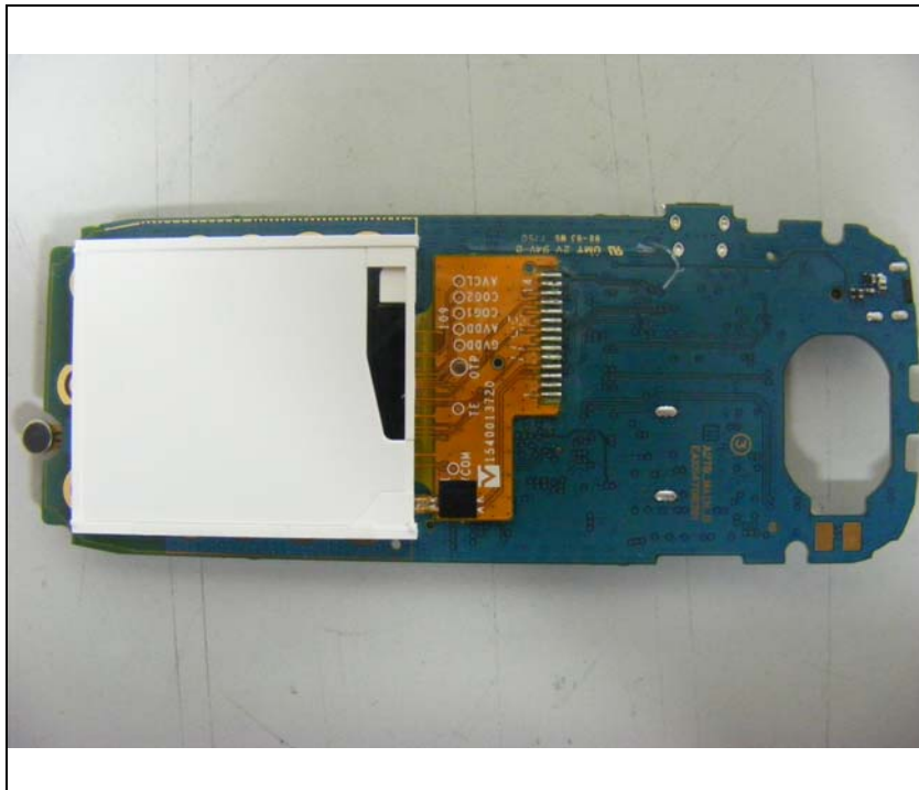
Top view of main board (Bottom of LCD module)
