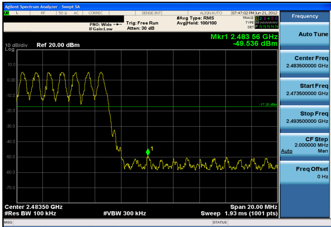
Plot 6-13. Band Edge Plot (Bluetooth with Hopping Enabled, 2Mbps)
