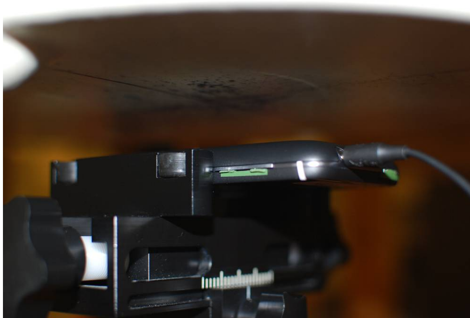
SAR Test Setup Photo 11 – Body-Worn Back at 2.0 cm
