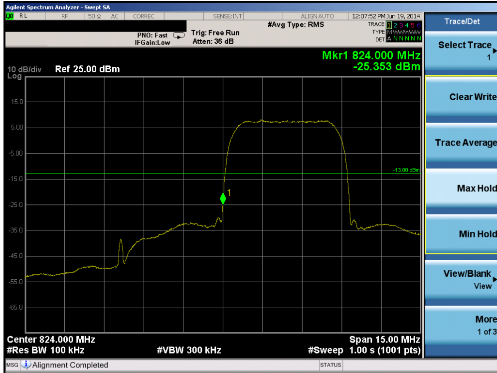
Plot 6-36. Band Edge Plot (Cellular WCDMA Mode – Ch. 4132)
