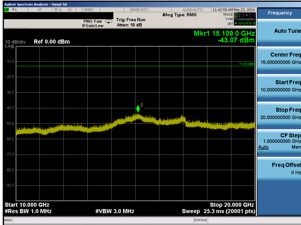
Plot 6-31. Conducted Spurious Plot (PCS WCDMA Mode – Ch. 9538)
