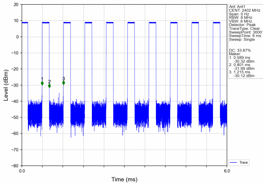
2M_LCH_2402MHz_Ant1_NTNV
