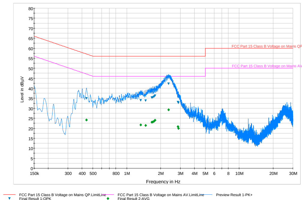
Plot 6-23. Line-Conducted Test Plot (L1)
