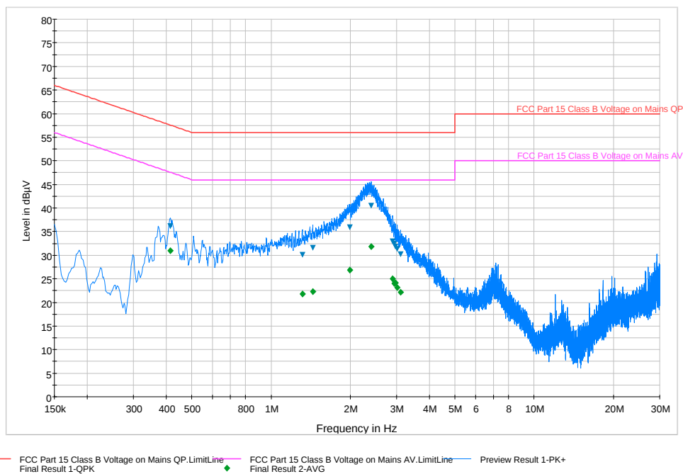
Plot 6-24. Line-Conducted Test Plot (N)
