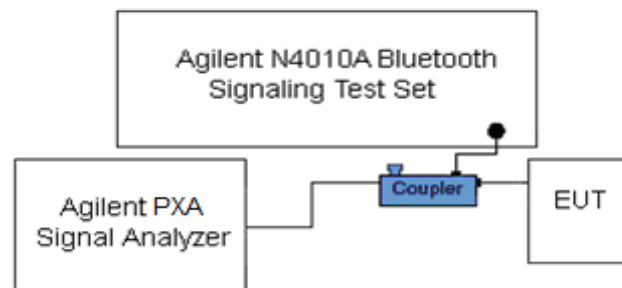
Figure 6-2. Test Instrument & Measurement Setup
