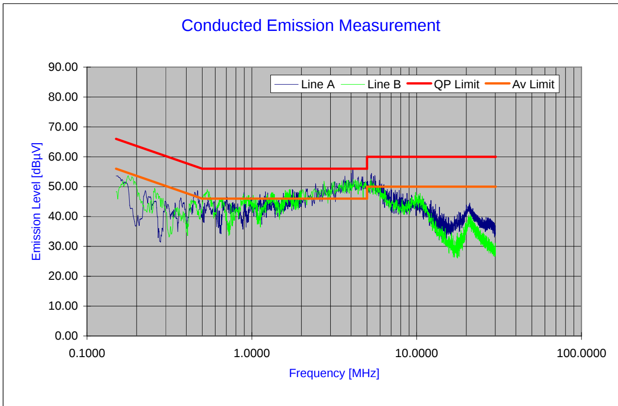
Plot 6-33. Line Conducted Plot with 802.11n
