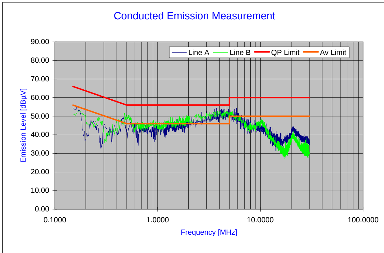
Plot 6-32. Line Conducted Plot with 802.11g
