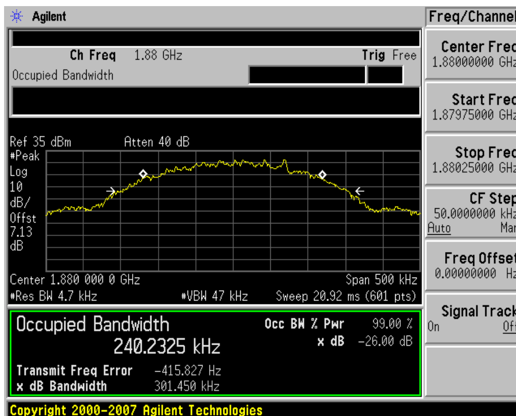
Plot 7-16. Occupied Bandwidth Plot (PCS GSM Mode – Ch. 661)
