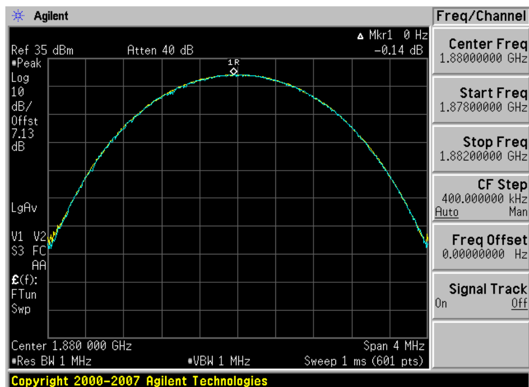
Plot 7-22. Peak-Average Ratio Plot (EDGE1900 Mode – Ch. 661)
