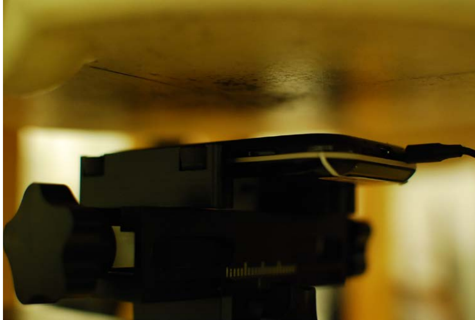
SAR Test Setup Photo 11: Body Worn at 2.0 cm
