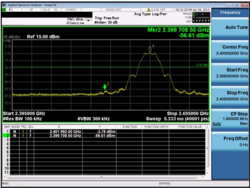
Low Band-edge
