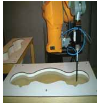
Figure 3.9 Simulated Tissue
