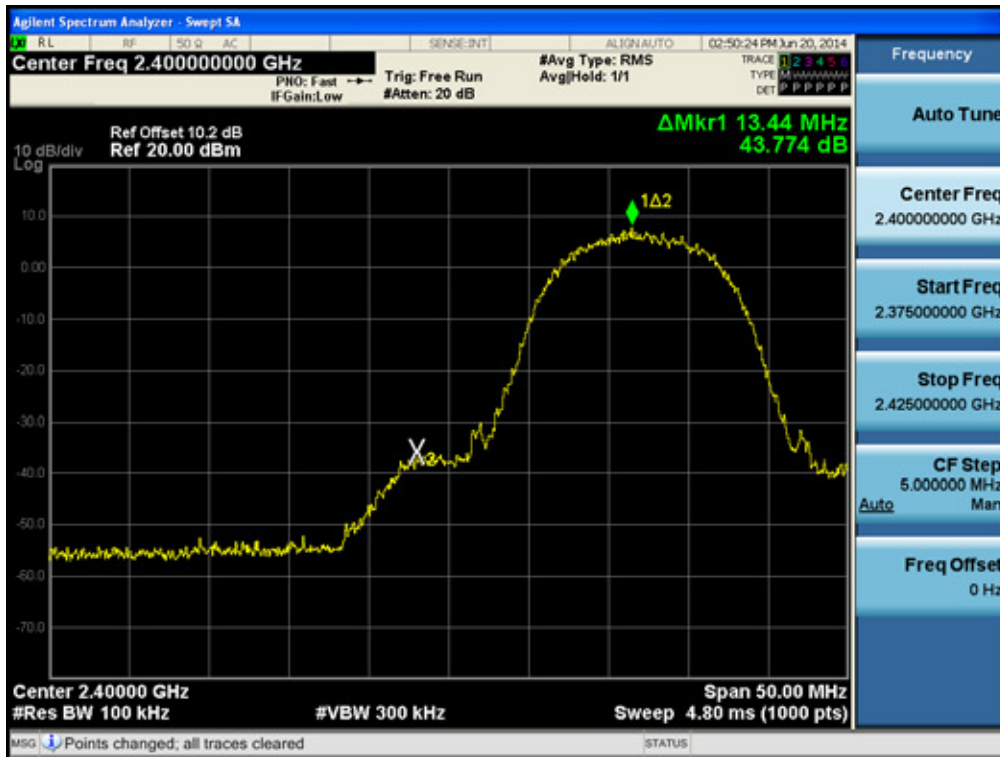
BandEdge (802.11b-CH1)
