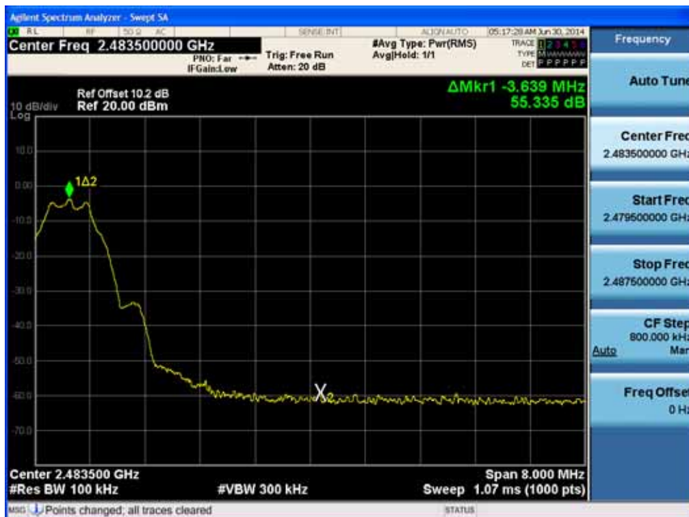
BandEdge (High-CH 39)
