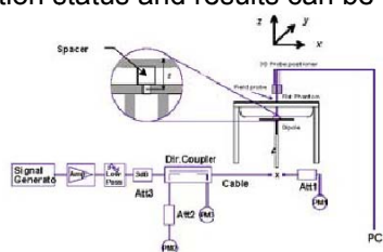
Figure 11.1 Dipole Verification Test Setup
