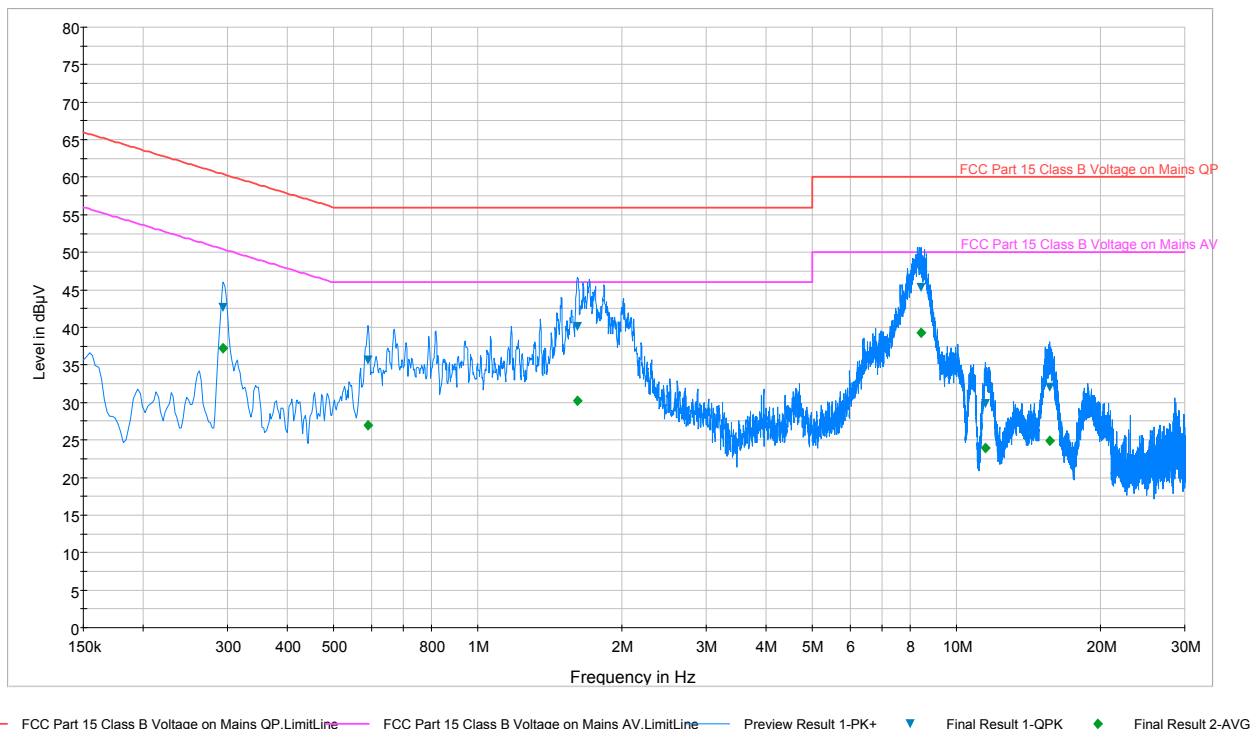
Plot 6-20. Line Conducted Plot with Bluetooth LE (L1)
