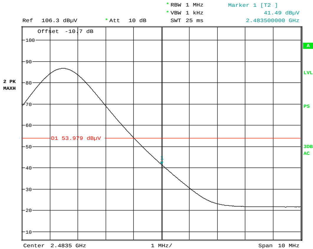
Plot 6-1. Radiated Restricted Upper Band Edge Measurement (Average)
