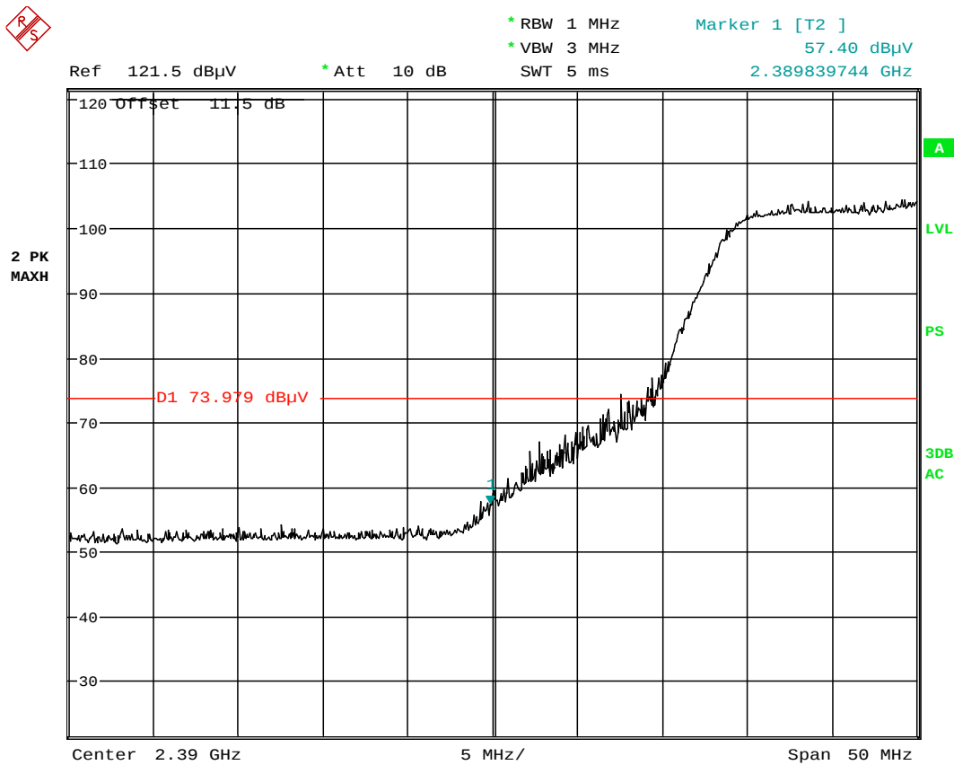
Plot 6-2. Radiated Restricted Lower Band Edge Measurement (Peak)
