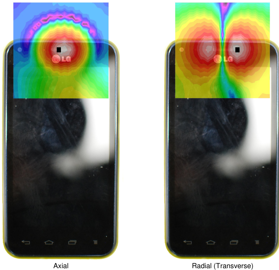
Figure 13-3 T-Coil Scan Overlay Magnetic Field Distributions
