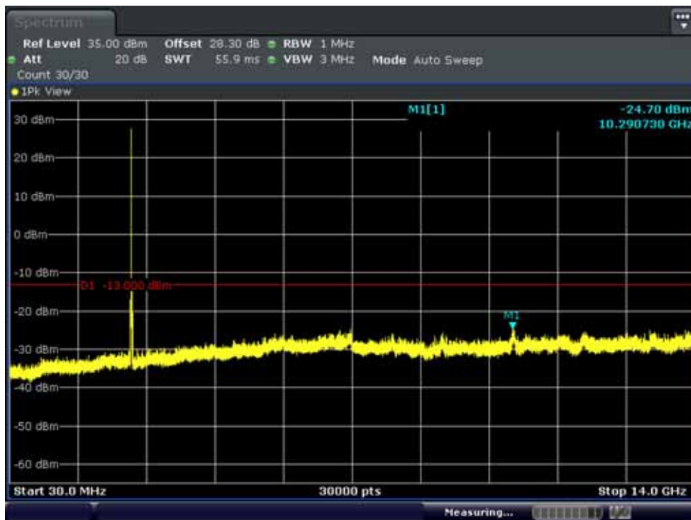
Conducted Spurious Plot 1 (20MHz Ch.20850 QPSK RF 1, Offset 0)
