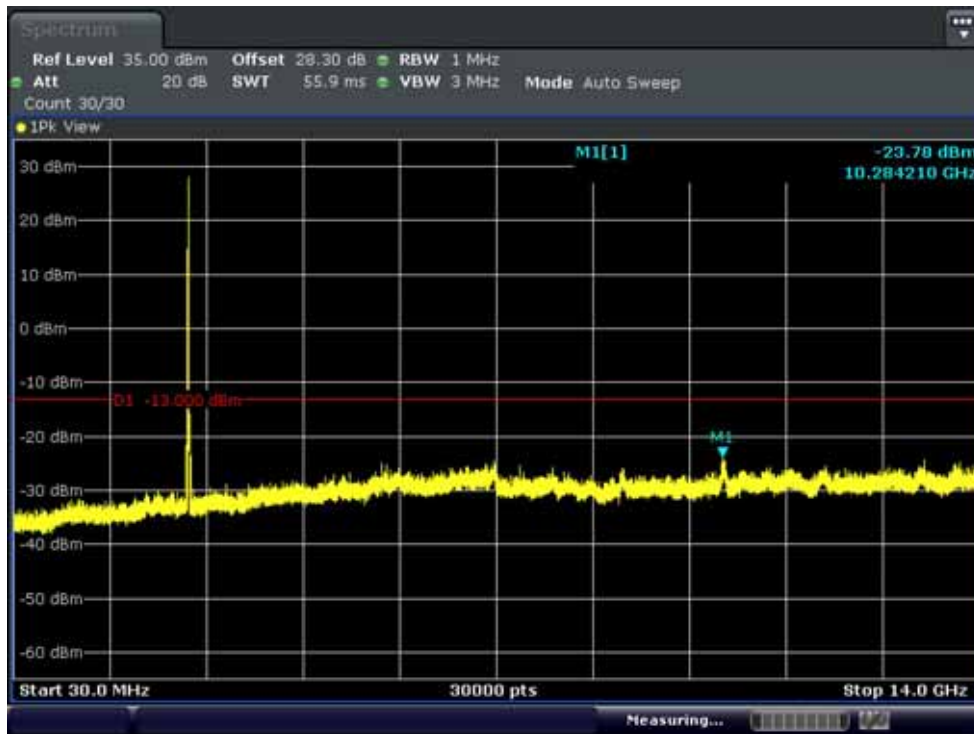
Conducted Spurious Plot 1 (20MHz Ch.21350 QPSK RF 1, Offset 0)
