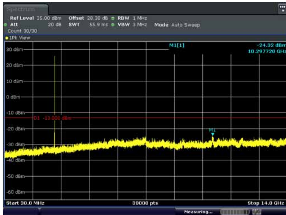
Conducted Spurious Plot 1 (5MHz Ch.20775 QPSK RF 1, Offset 0)
