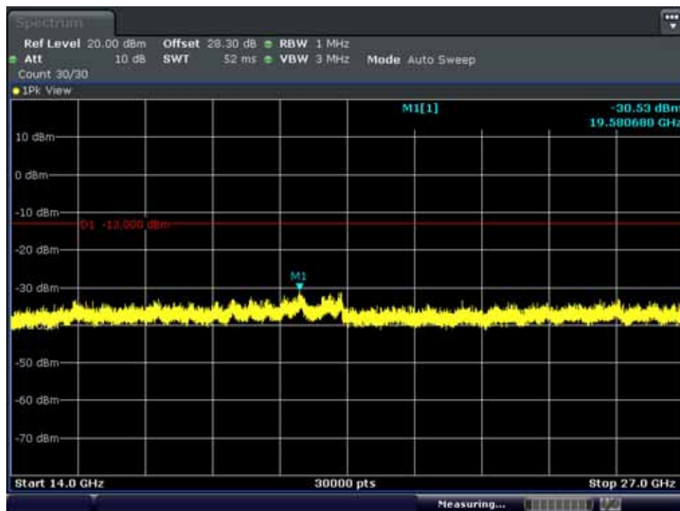
Conducted Spurious Plot 2 (5MHz Ch.20775 QPSK RF 1, Offset 0)
