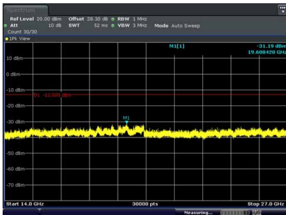
Conducted Spurious Plot 2 (10MHz Ch.21100 QPSK RF 1, Offset 0)
