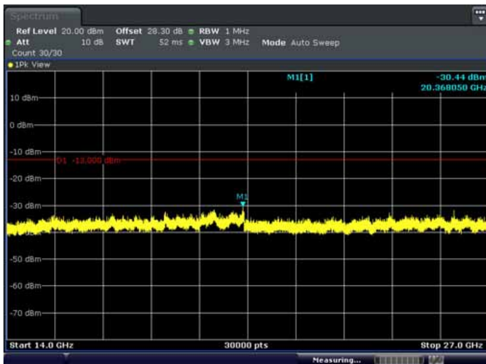
Conducted Spurious Plot 2 (20MHz Ch.20850 QPSK RF 1, Offset 0)
