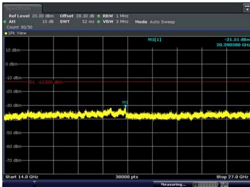
Conducted Spurious Plot 2 (5MHz Ch.21425 QPSK RF 1, Offset 0)
