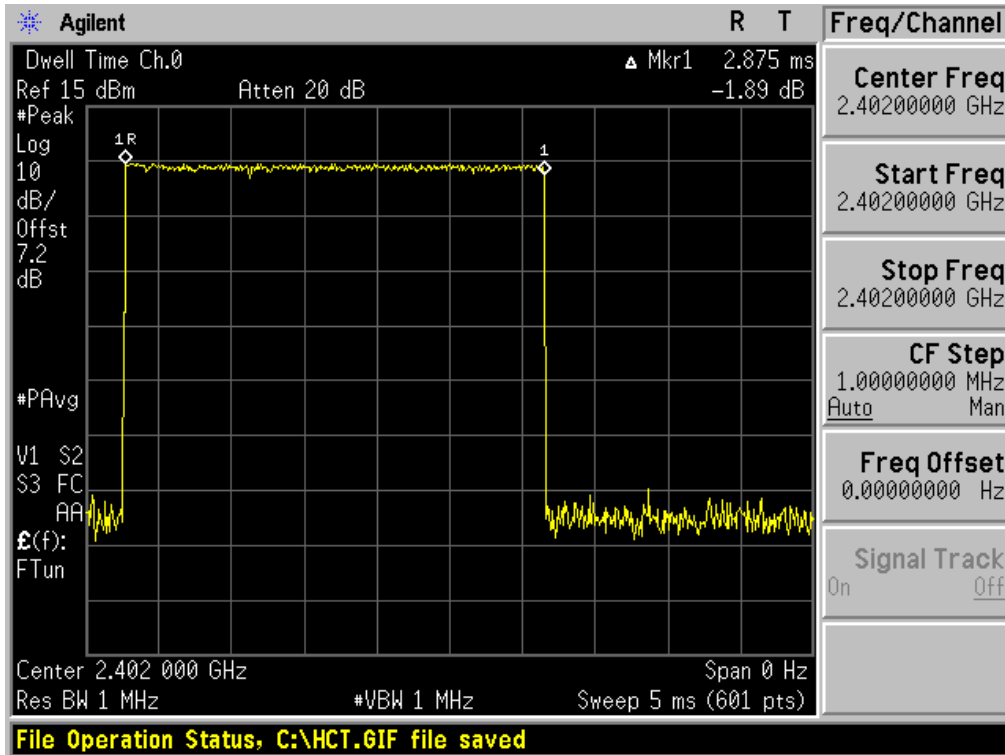
Test Plots ( \pi/4 DQPSK) Dwell Time (Low-CH)
