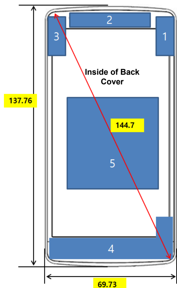
LG-D722J NFC Antenna Location
