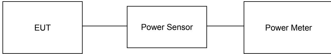
Figure 10.3 Average Power Measurement Setup for Bandwidths < 50 MHz
