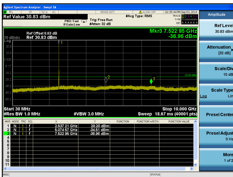
LTE Band 7 / 5 MHz / QPSK - RB Offset/Size (24/1) – Mid Channel
