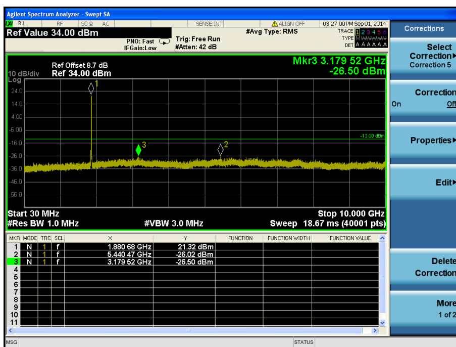
LTE Band 2 / 15 MHz / QPSK - RB Offset/Size (19/36) – Mid Channel
