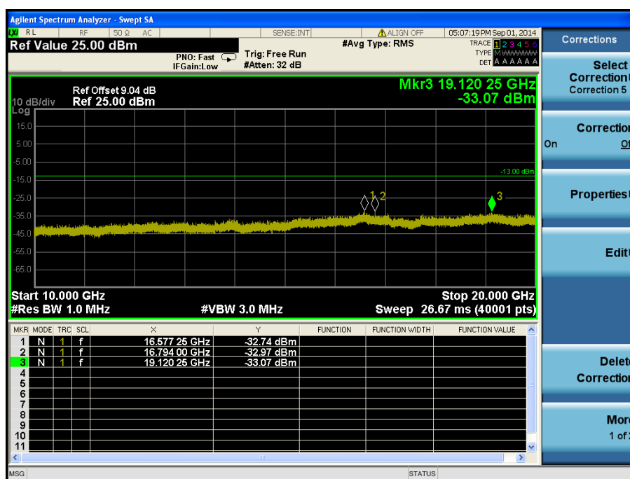
LTE Band 4 / 1.4 MHz / QPSK - RB Offset/Size (0/3) – Mid Channel
