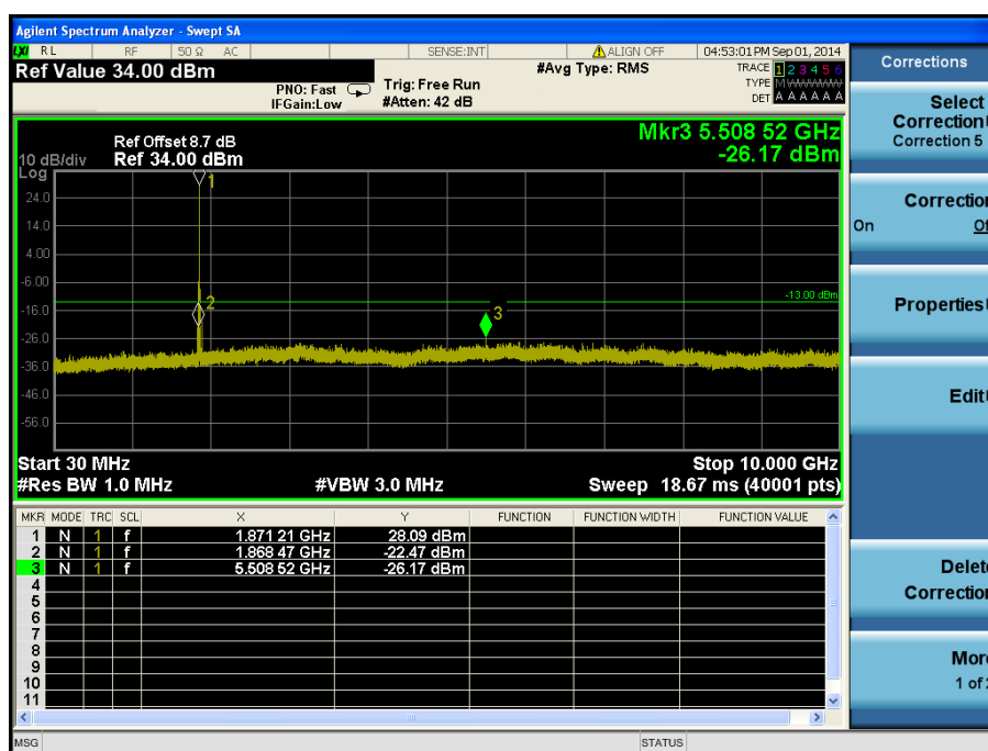
LTE Band 2 / 20 MHz / 16QAM - RB Offset/Size (0/1) – Mid Channel
