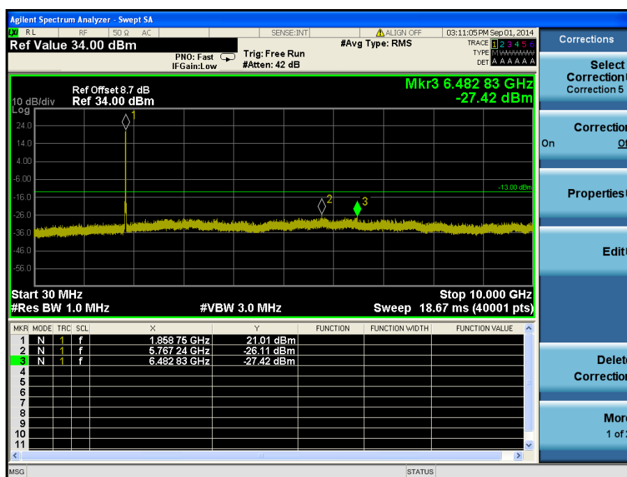
LTE Band 2 / 10 MHz / QPSK - RB Offset/Size (0/50) – Low Channel
