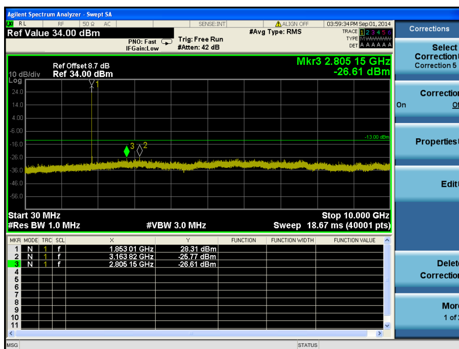
LTE Band 2 / 3 MHz / 16QAM - RB Offset/Size (14/1) – Low Channel
