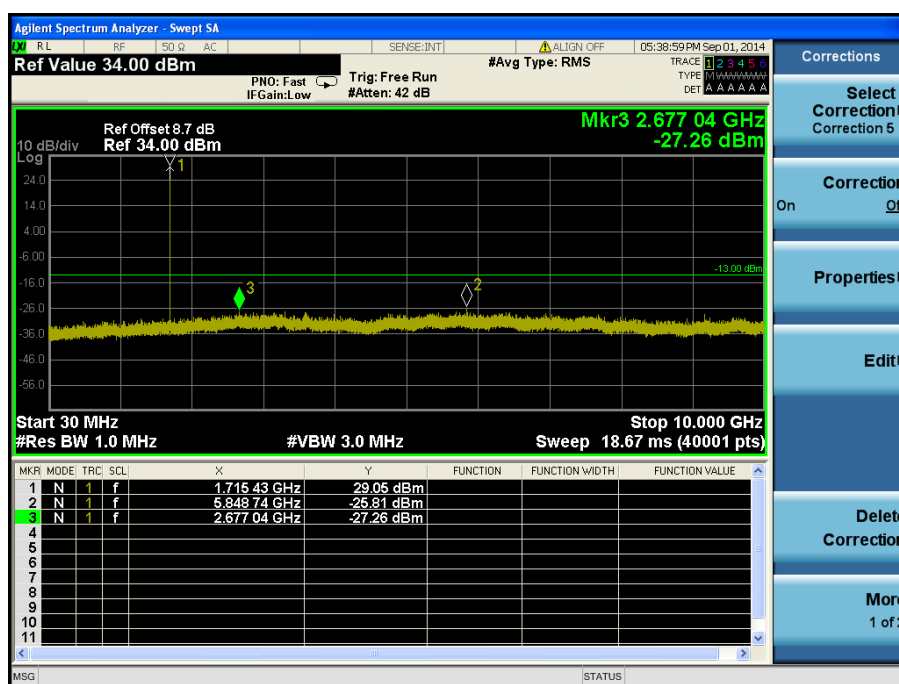
LTE Band 4 / 10 MHz / QPSK - RB Offset/Size (25/1) – Low Channel
