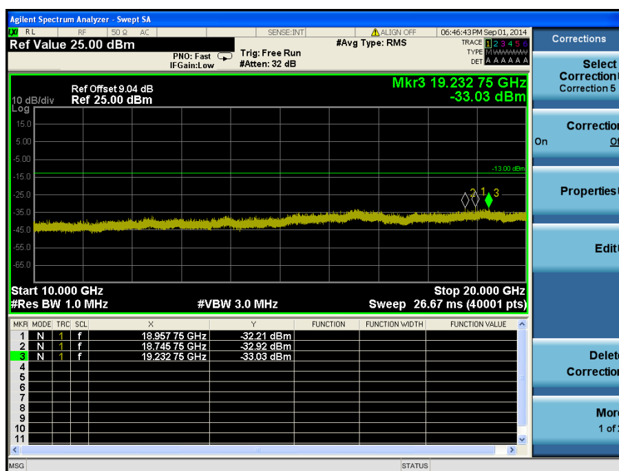
LTE Band 4 / 5 MHz / 16QAM - RB Offset/Size (0/12) – High Channel
