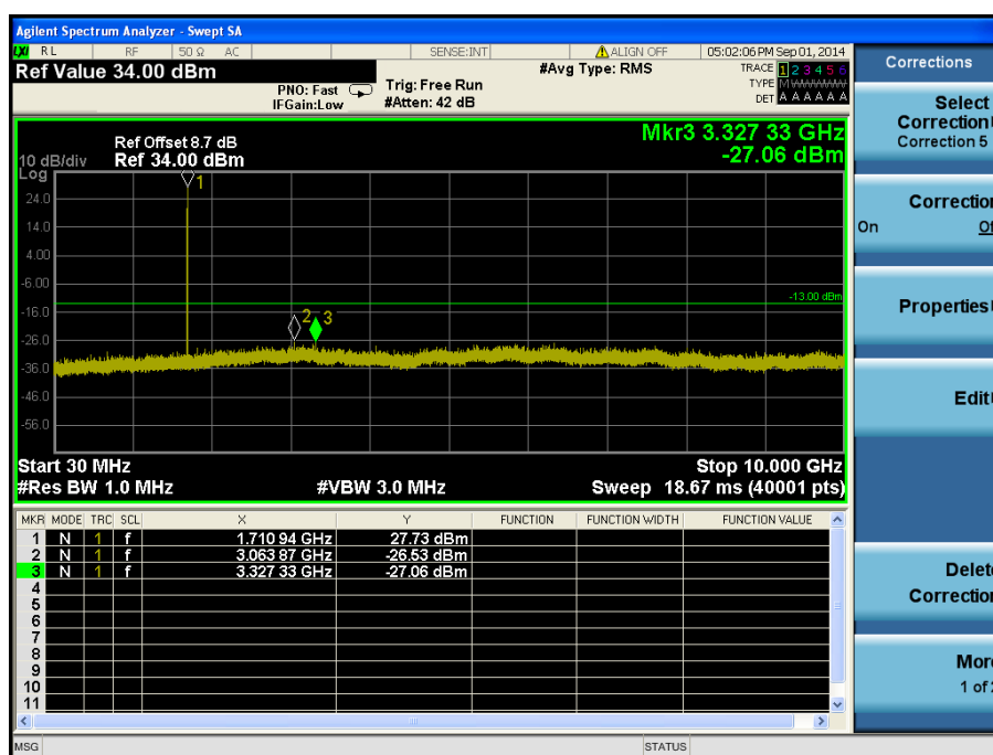
LTE Band 4 / 1.4 MHz / QPSK - RB Offset/Size (3/1) – Low Channel
