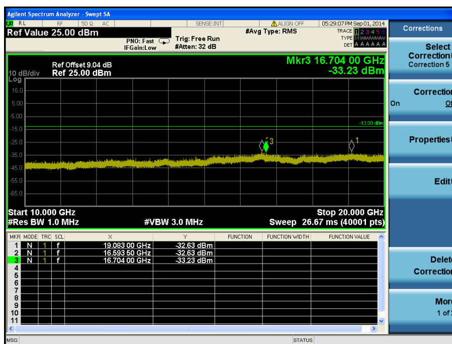
LTE Band 4 / 5 MHz / QPSK - RB Offset/Size (13/12) – Low Channel
