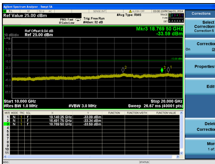
LTE Band 2 / 5 MHz / QPSK - RB Offset/Size (12/1) – Mid Channel
