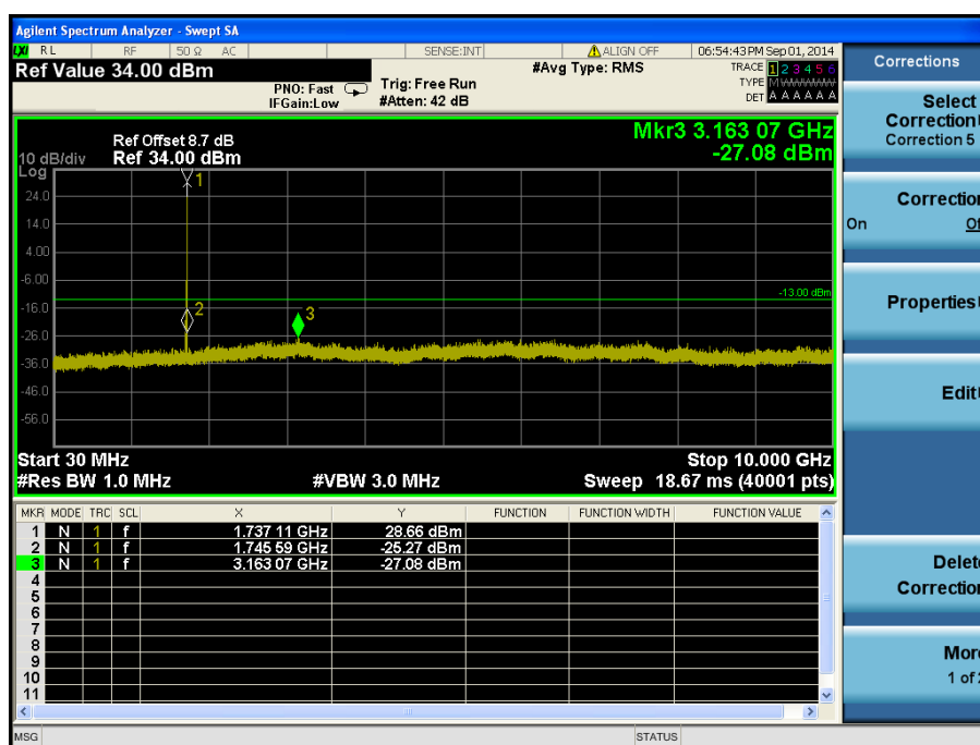
LTE Band 4 / 10 MHz / 16QAM - RB Offset/Size (49/1) – Mid Channel
