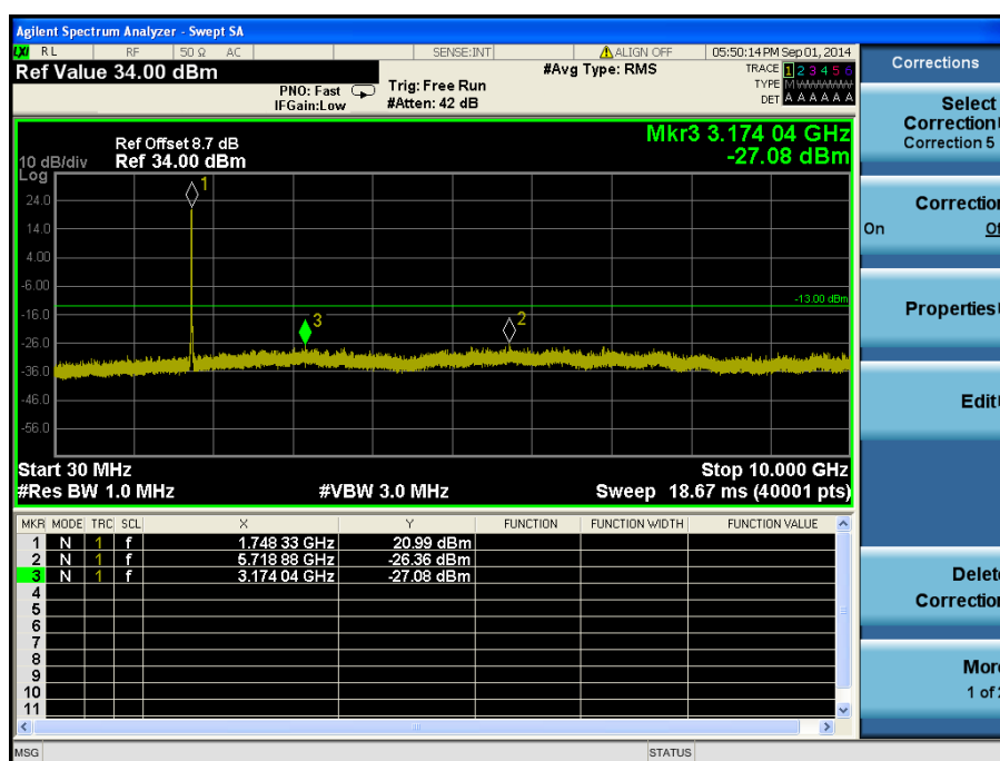
LTE Band 4 / 10 MHz / QPSK - RB Offset/Size (0/50) – High Channel
