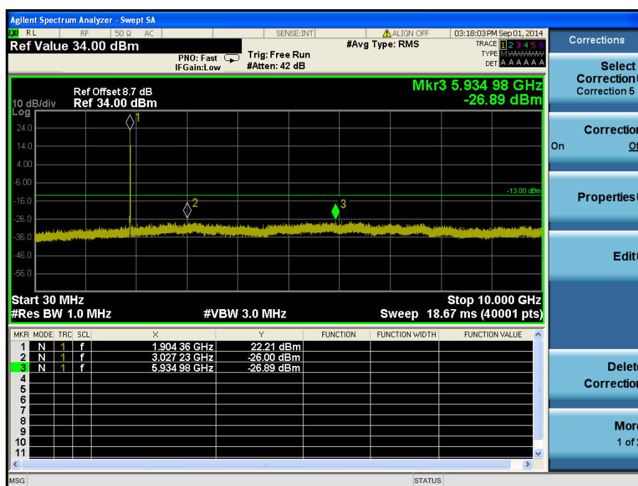
LTE Band 2 / 10 MHz / QPSK - RB Offset/Size (0/25) – High Channel
