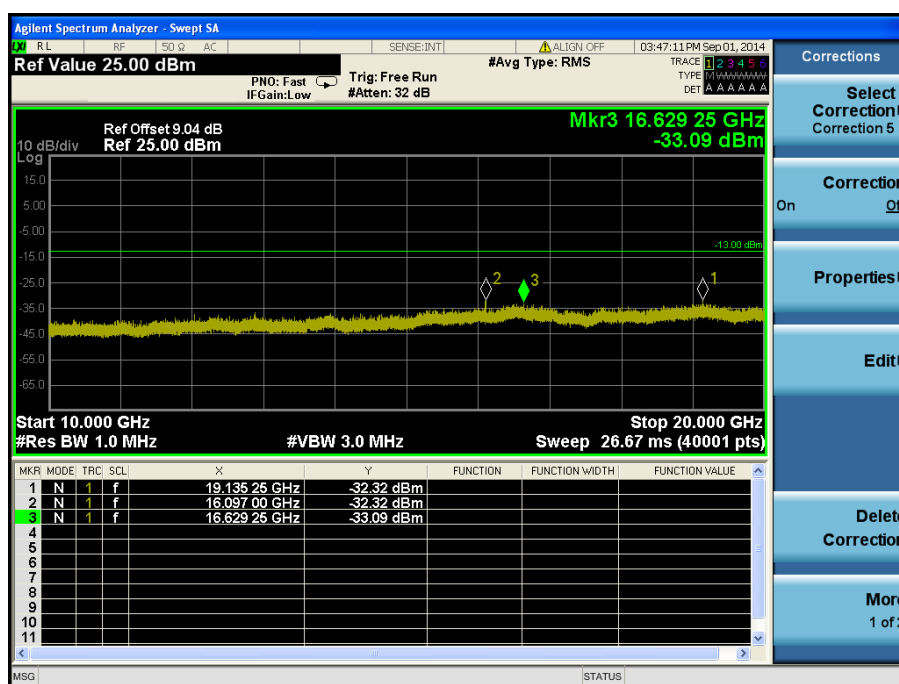
LTE Band 2 / 1.4 MHz / 16QAM - RB Offset/Size (3/1) – Low Channel
