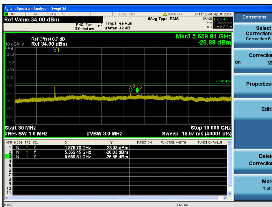
LTE Band 2 / 10 MHz / QPSK - RB Offset/Size (0/1) – Mid Channel
