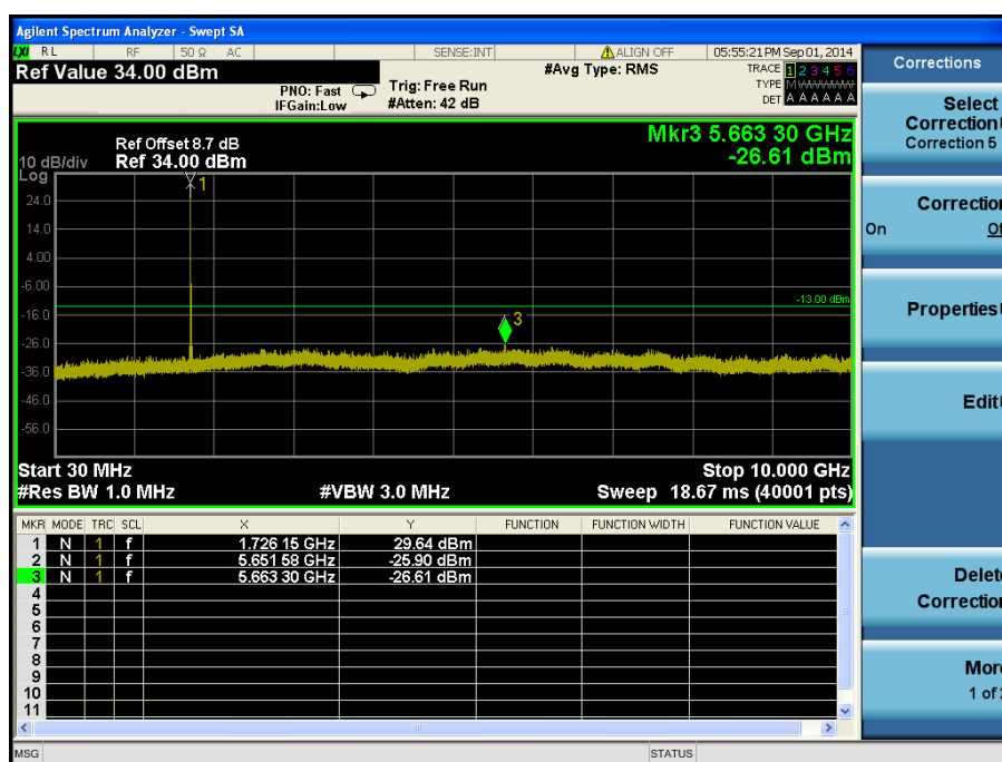
LTE Band 4 / 15 MHz / QPSK - RB Offset/Size (0/1) – Mid Channel
