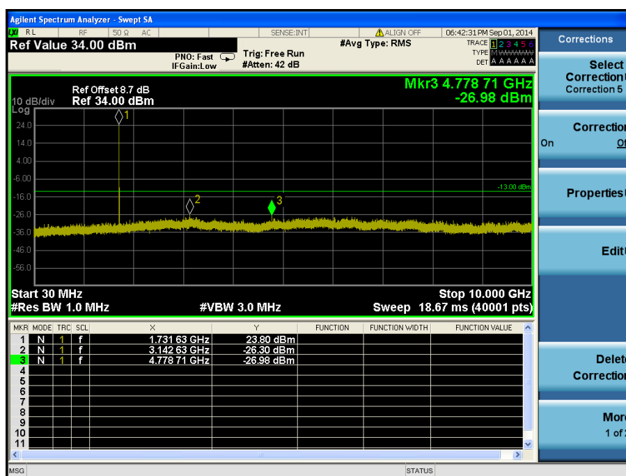
LTE Band 4 / 5 MHz / 16QAM - RB Offset/Size (0/12) – Mid Channel
