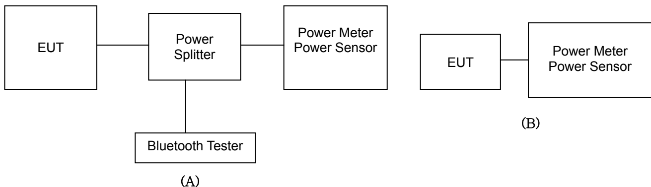
Figure 10.4 Power Measurement Setup
