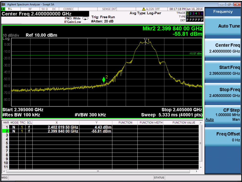
Low Band-edge
