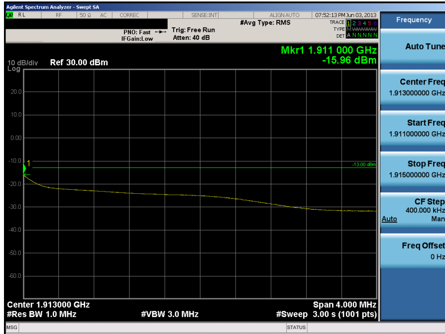
Plot 7-58. 4MHz Span Plot (PCS WCDMA Mode – Ch. 9538)
