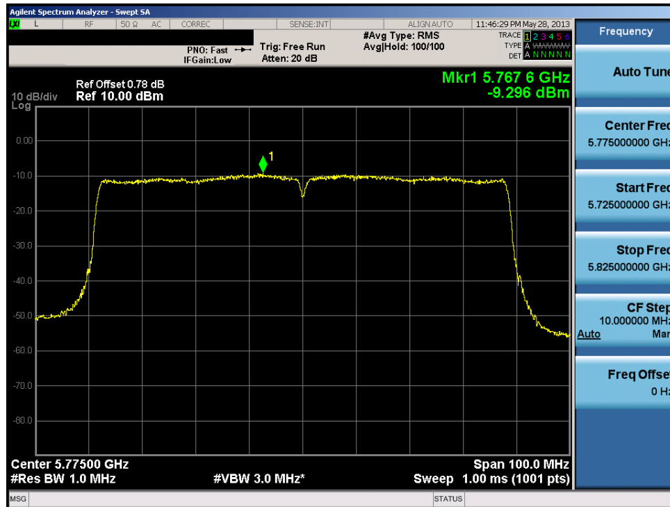
Plot 6-77. Peak Power Spectral Density Plot (80MHz BW 802.11ac (UNII Band 4) – Ch. 155)
