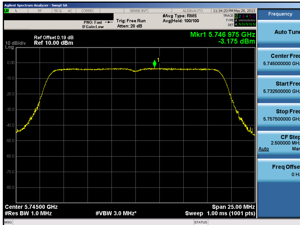
Plot 6-72. Peak Power Spectral Density Plot (20MHz BW 802.11n (UNII Band 4) – Ch. 149)
