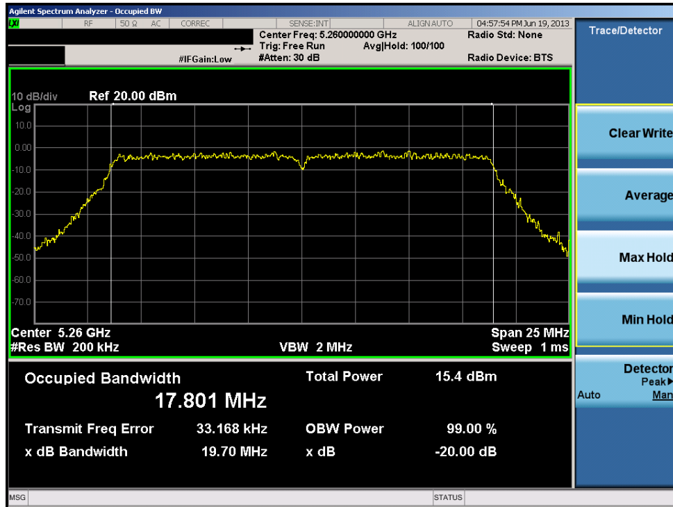
Plot 6-39. 20dB Bandwidth Plot (20MHz BW 802.11n (UNII Band 2) – Ch. 52)
