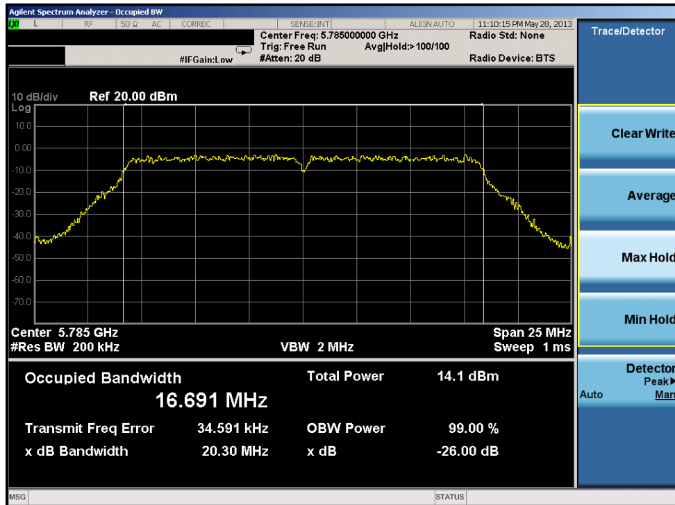
Plot 6-30. 26dB Bandwidth Plot (802.11a (UNII Band 4) – Ch. 157)
