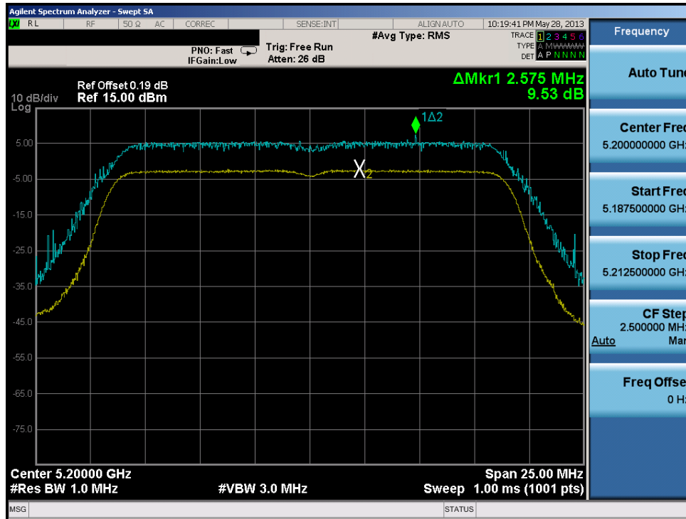
Plot 6-79. Peak Excursion Ratio Plot (20MHz BW 802.11n)
