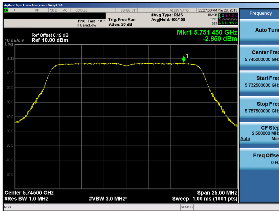
Plot 6-69. Peak Power Spectral Density Plot (802.11a (UNII Band 4) – Ch. 149)
