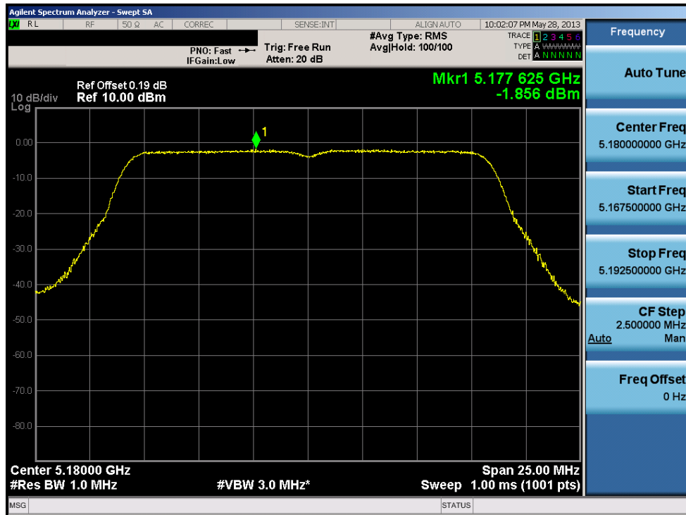
Plot 6-41. Peak Power Spectral Density Plot (802.11a (UNII Band 1) – Ch. 36)
