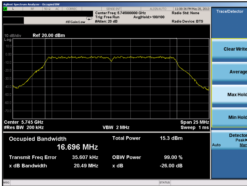
Plot 6-29. 26dB Bandwidth Plot (802.11a (UNII Band 4) – Ch. 149)
