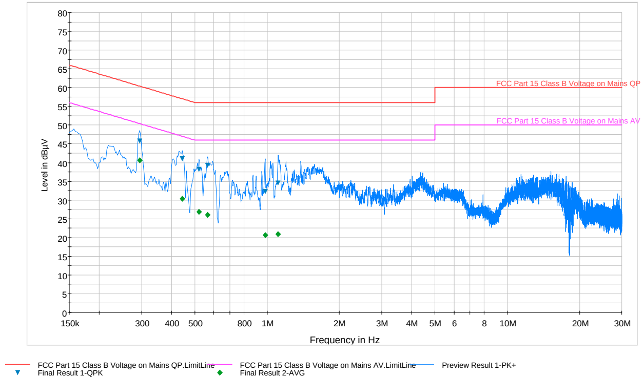
Plot 6-106. Line Conducted Plot with 802.11a UNII Band 2 (N)
