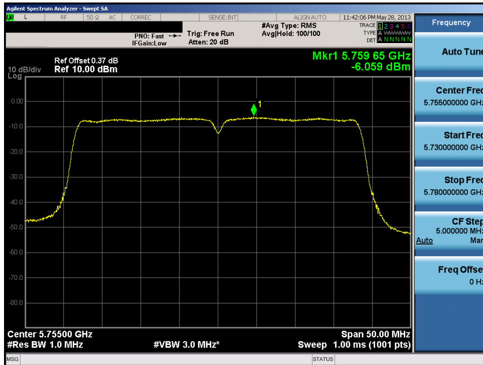
Plot 6-75. Peak Power Spectral Density Plot (40MHz BW 802.11n (UNII Band 4) – Ch. 151)
