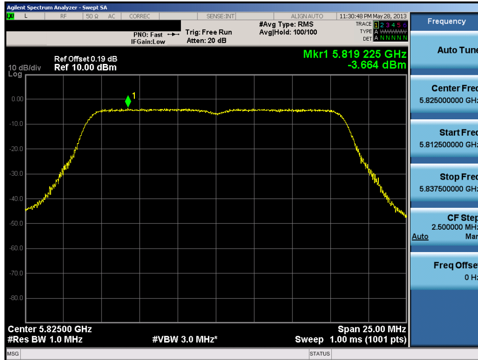
Plot 6-71. Peak Power Spectral Density Plot (802.11a (UNII Band 4) – Ch. 165)
