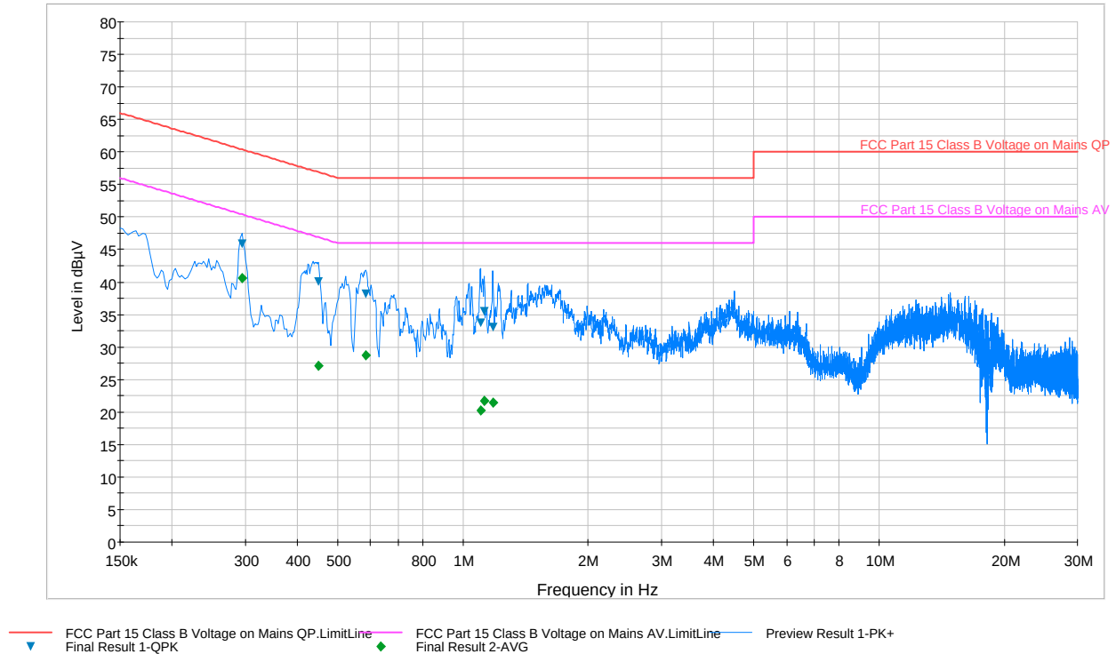
Plot 6-104. Line Conducted Plot with 802.11a UNII Band 1 (N)
