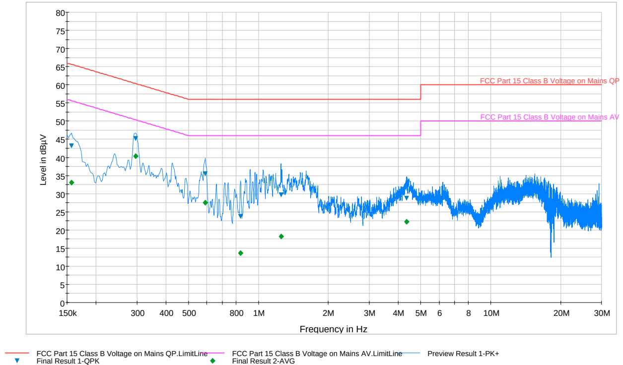
Plot 6-105. Line Conducted Plot with 802.11a UNII Band 2 (L1)
