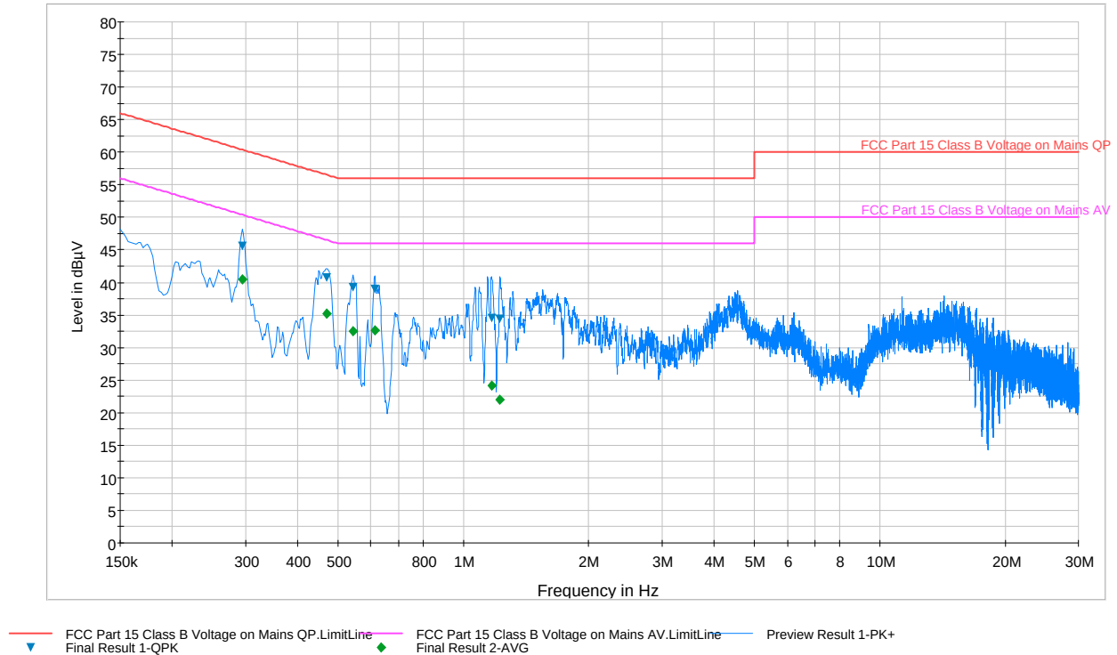
Plot 6-108. Line Conducted Plot with 802.11a UNII Band 3 (N)
