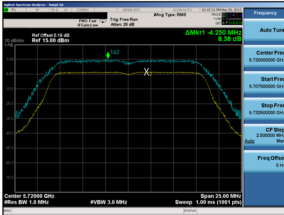
Plot 6-78. Peak Excursion Ratio Plot (802.11a)
