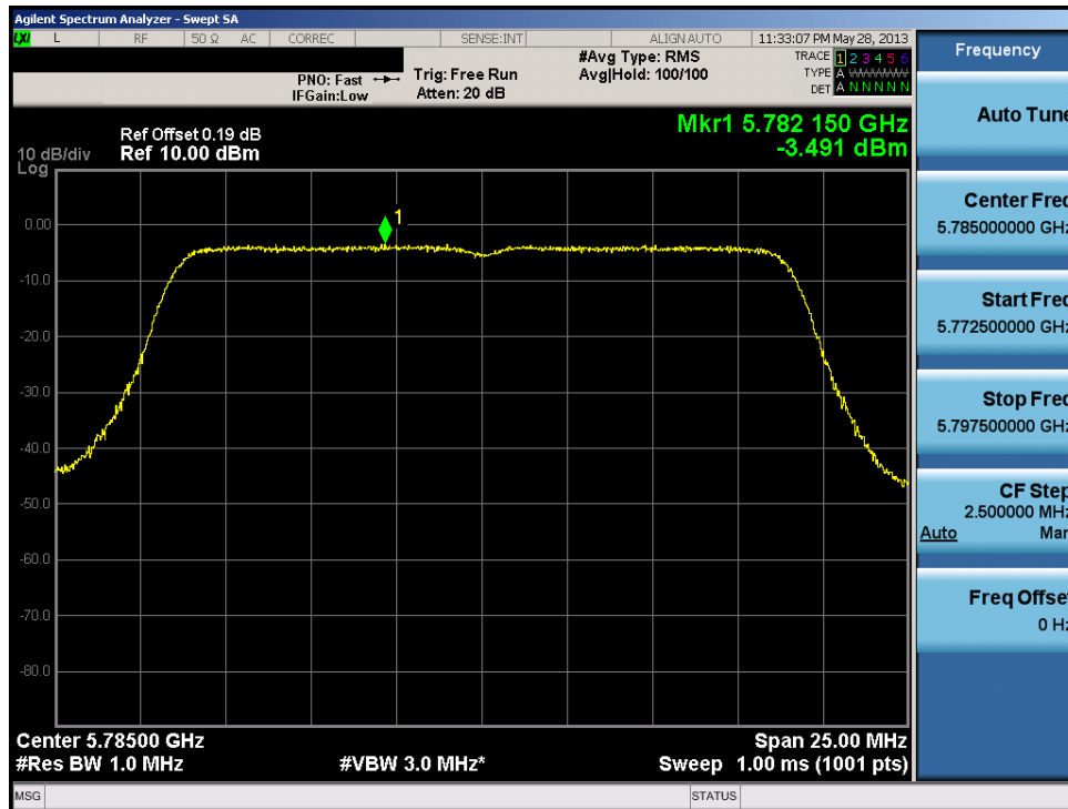
Plot 6-73. Peak Power Spectral Density Plot (20MHz BW 802.11n (UNII Band 4) – Ch. 157)
