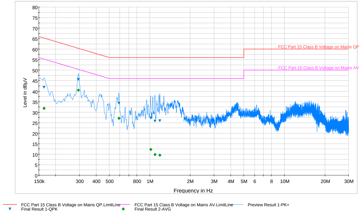
Plot 6-107. Line Conducted Plot with 802.11a UNII Band 3 (L1)
