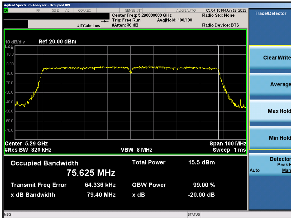
Plot 6-40. 20dB Bandwidth Plot (80MHz BW 802.11ac (UNII Band 2) – Ch. 58)
