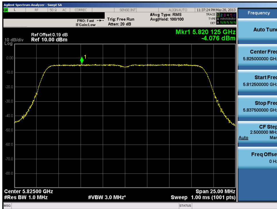
Plot 6-74. Peak Power Spectral Density Plot (20MHz BW 802.11n (UNII Band 4) – Ch. 165)
