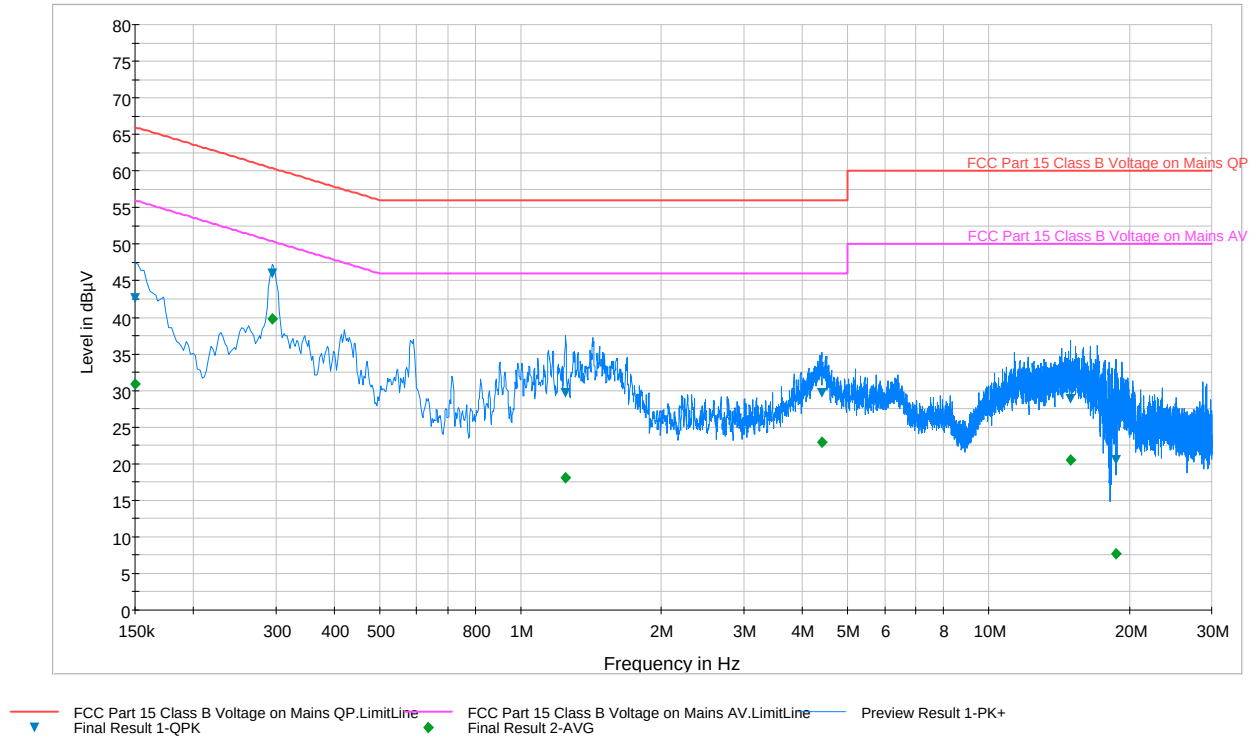
Plot 6-109. Line Conducted Plot with 802.11a UNII Band 4 (L1)
