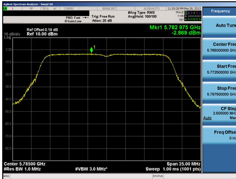
Plot 6-70. Peak Power Spectral Density Plot (802.11a (UNII Band 4) – Ch. 157)
