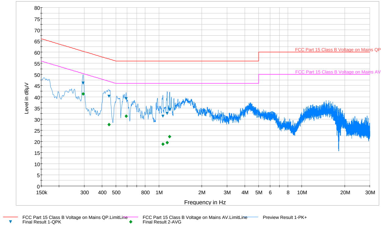
Plot 6-110. Line Conducted Plot with 802.11a UNII Band 4 (N)
