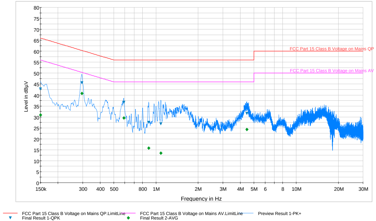
Plot 6-103. Line Conducted Plot with 802.11a UNII Band 1 (L1)
