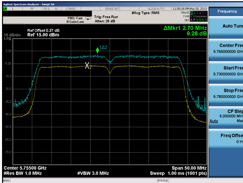
Plot 6-80. Peak Excursion Ratio Plot (40MHz BW 802.11n)
