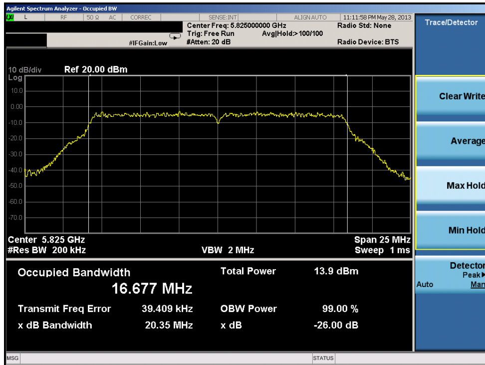
Plot 6-31. 26dB Bandwidth Plot (802.11a (UNII Band 4) – Ch. 165)
