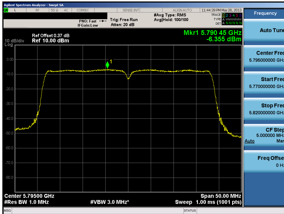
Plot 6-76. Peak Power Spectral Density Plot (40MHz BW 802.11n (UNII Band 4) – Ch. 159)
