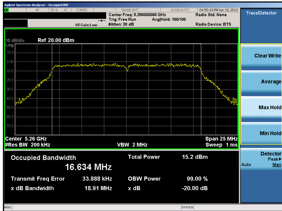
Plot 6-38. 20dB Bandwidth Plot (20MHz BW 802.11a (UNII Band 2) – Ch. 52)
