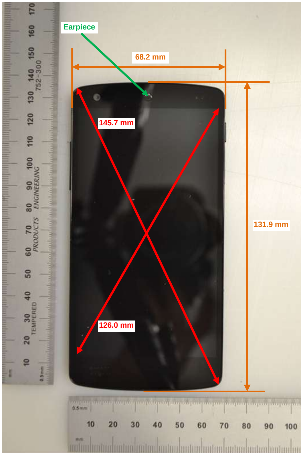
Overall Dimensions
