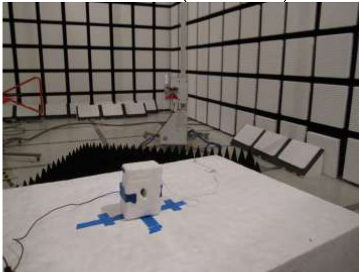
RADIATED BACK PHOTO (ABOVE 1 GHz)
