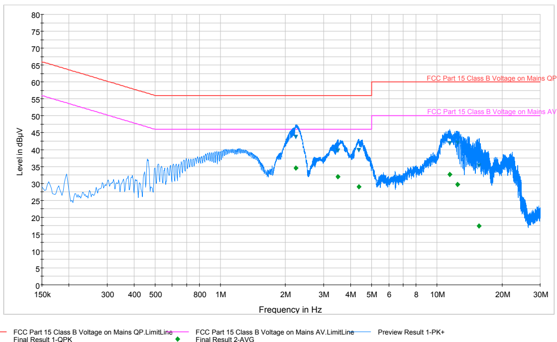
Plot 6-23. Line Conducted Plot with Bluetooth LE (N)
