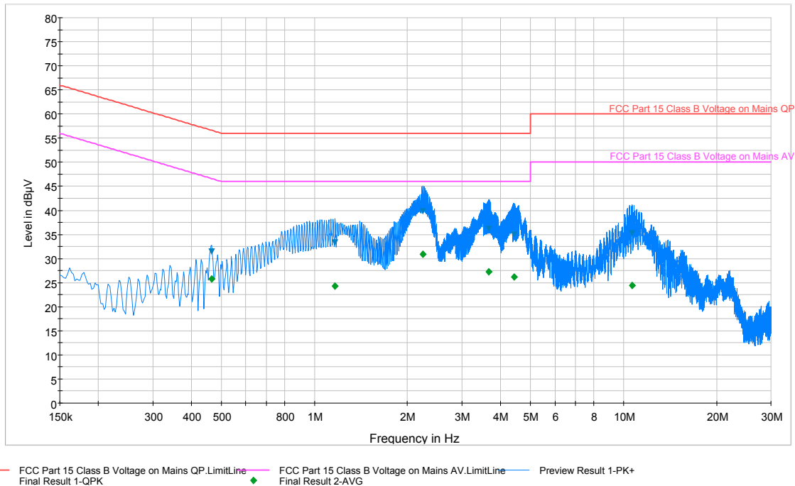
Plot 6-22. Line Conducted Plot with Bluetooth LE (L1)
