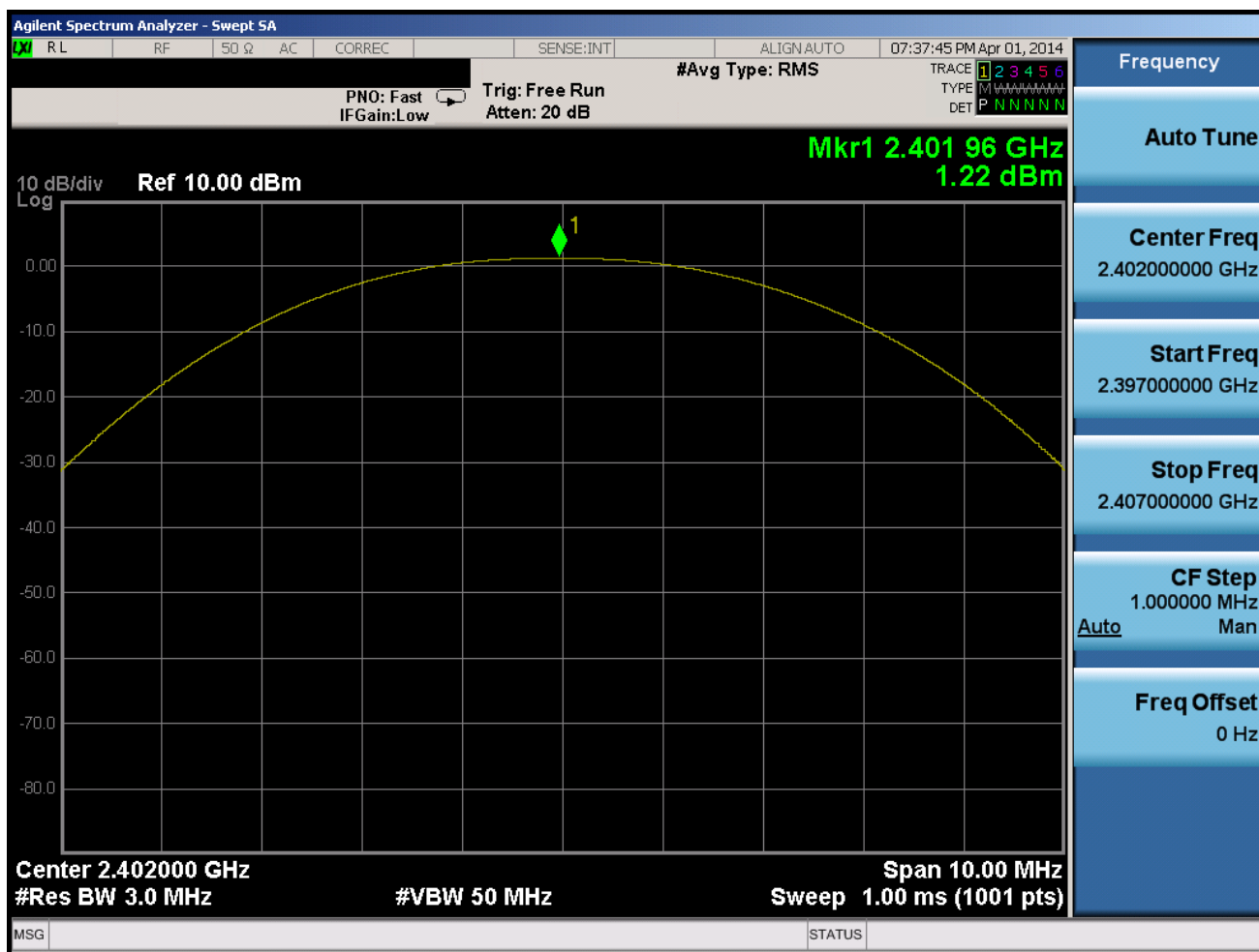
Plot 6-4. Peak Power Plot (Bluetooth (LE) – Ch. 0)
