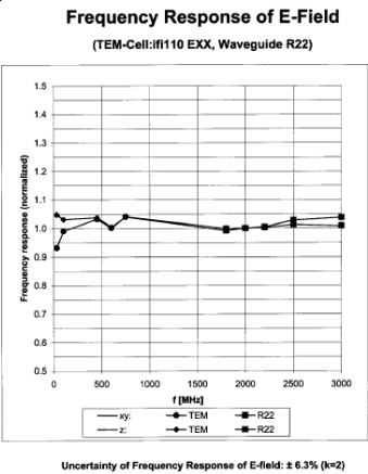
Figure 5-2 E-Field Probe Frequency Response
