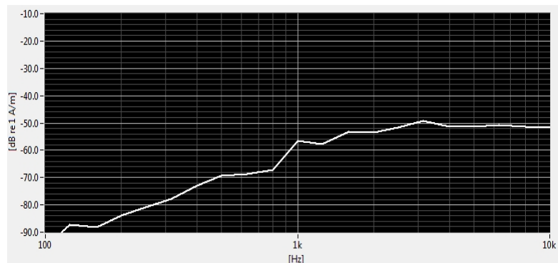
Figure 7-2 Worst-case ABM2 Plot for WD
