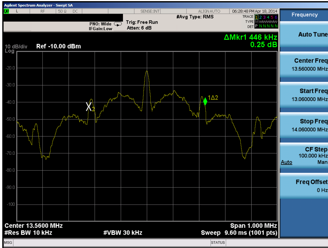
Figure 8-3. WCC 20dB Bandwidth Plot
