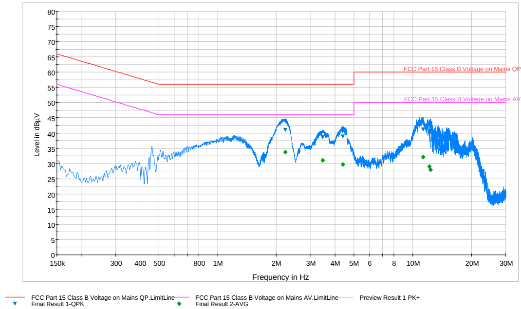
Plot 6-98. Line Conducted Plot with 802.11a UNII Band 2C (N)
