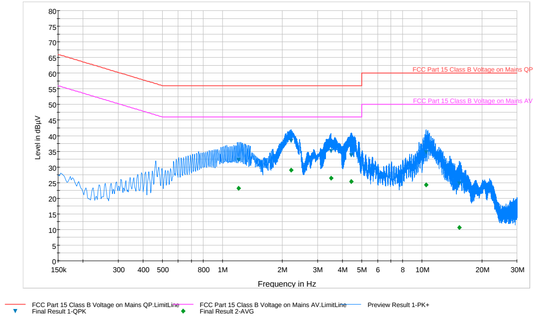
Plot 6-93. Line Conducted Plot with 802.11a UNII Band 1 (L1)
