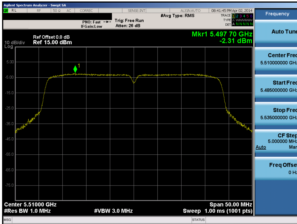
Plot 6-59. Peak Power Spectral Density Plot (40MHz BW 802.11n (UNII Band 2C) – Ch. 102)
