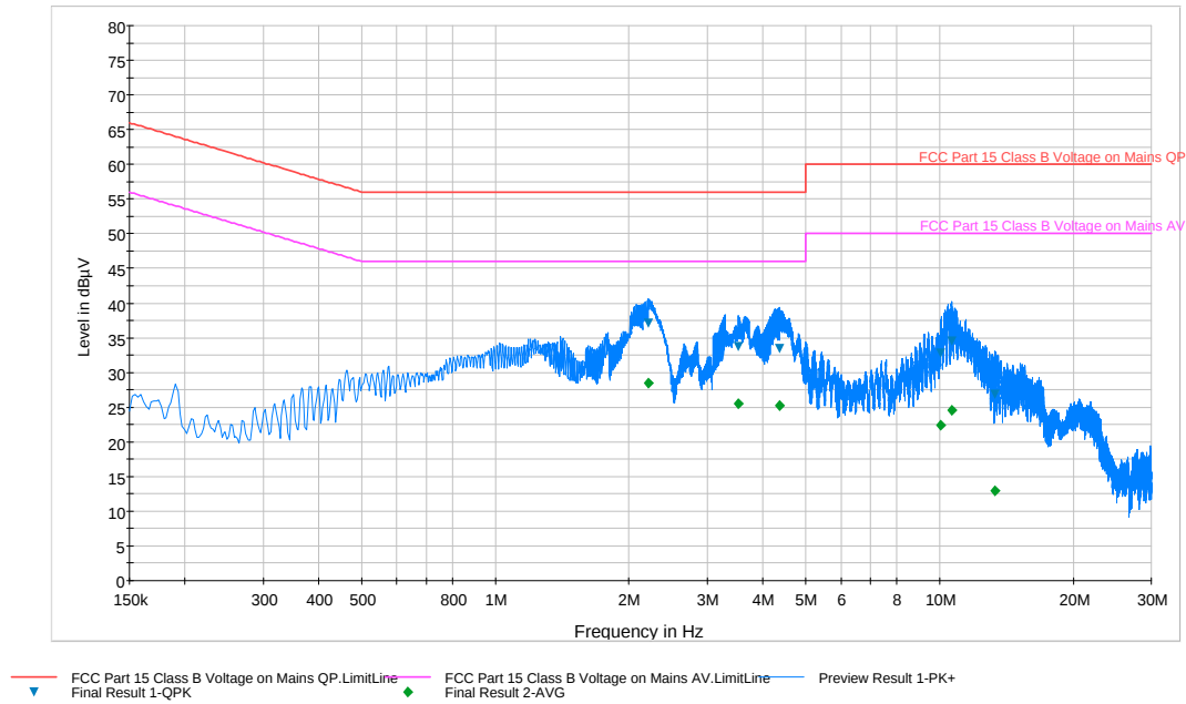
Plot 6-97. Line Conducted Plot with 802.11a UNII Band 2C (L1)
