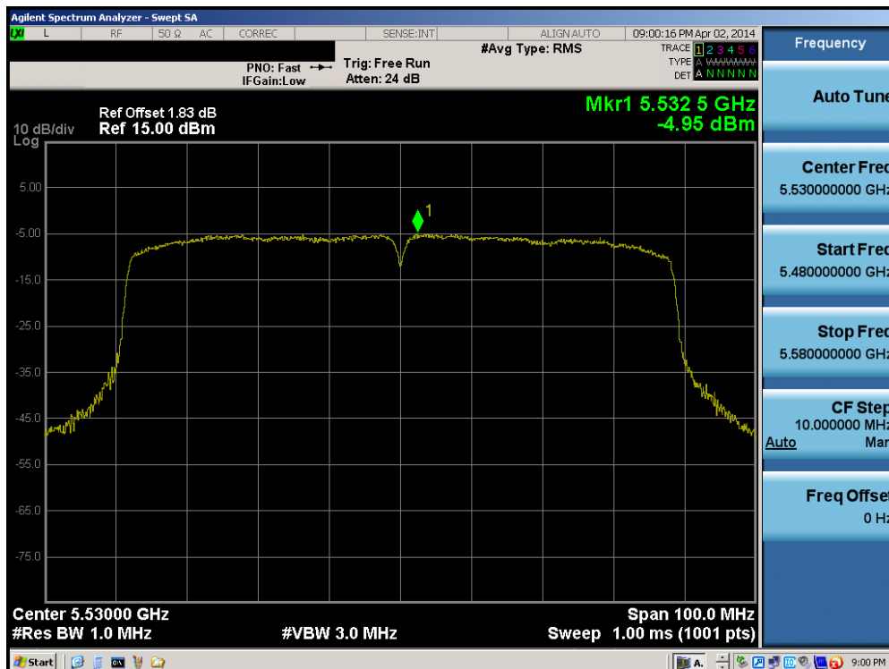
Plot 6-62. Peak Power Spectral Density Plot (80MHz BW 802.11ac (UNII Band 2C) – Ch. 106)
