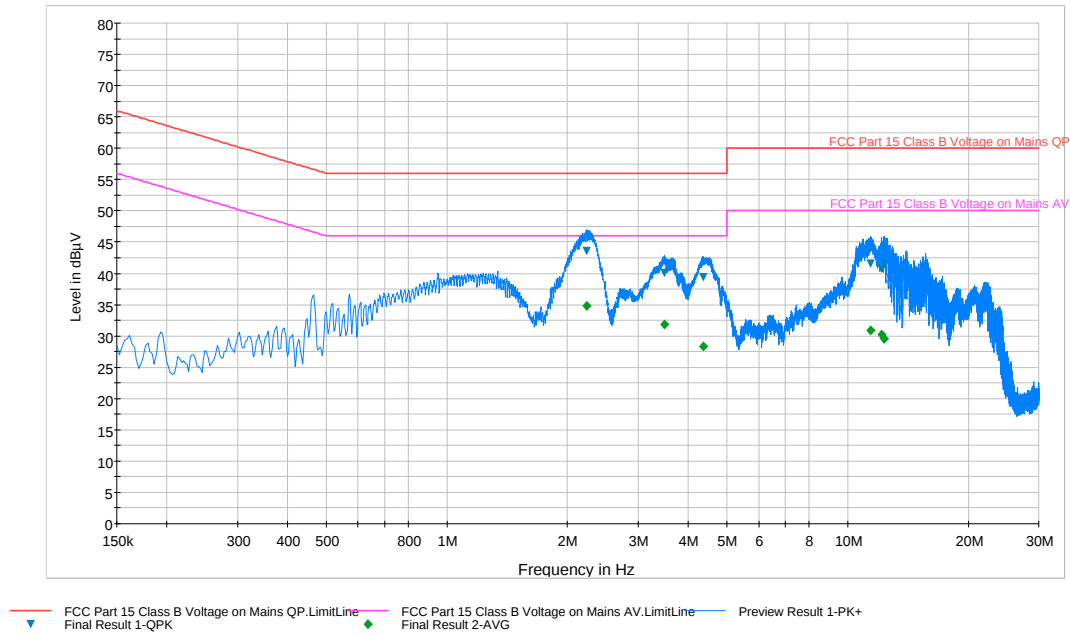
Plot 6-94. Line Conducted Plot with 802.11a UNII Band 1 (N)
