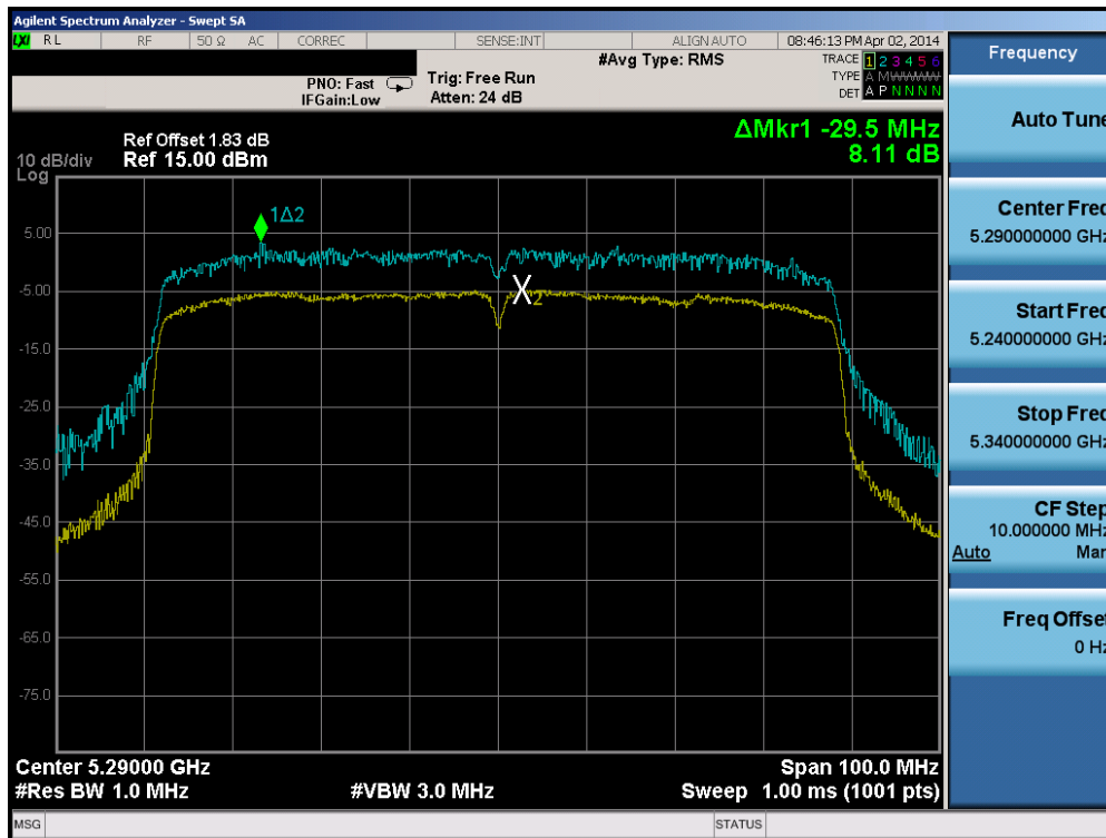
Plot 6-64. Peak Excursion Ratio Plot (80MHz BW 802.11ac (UNII Band 2A) – Ch. 58)
