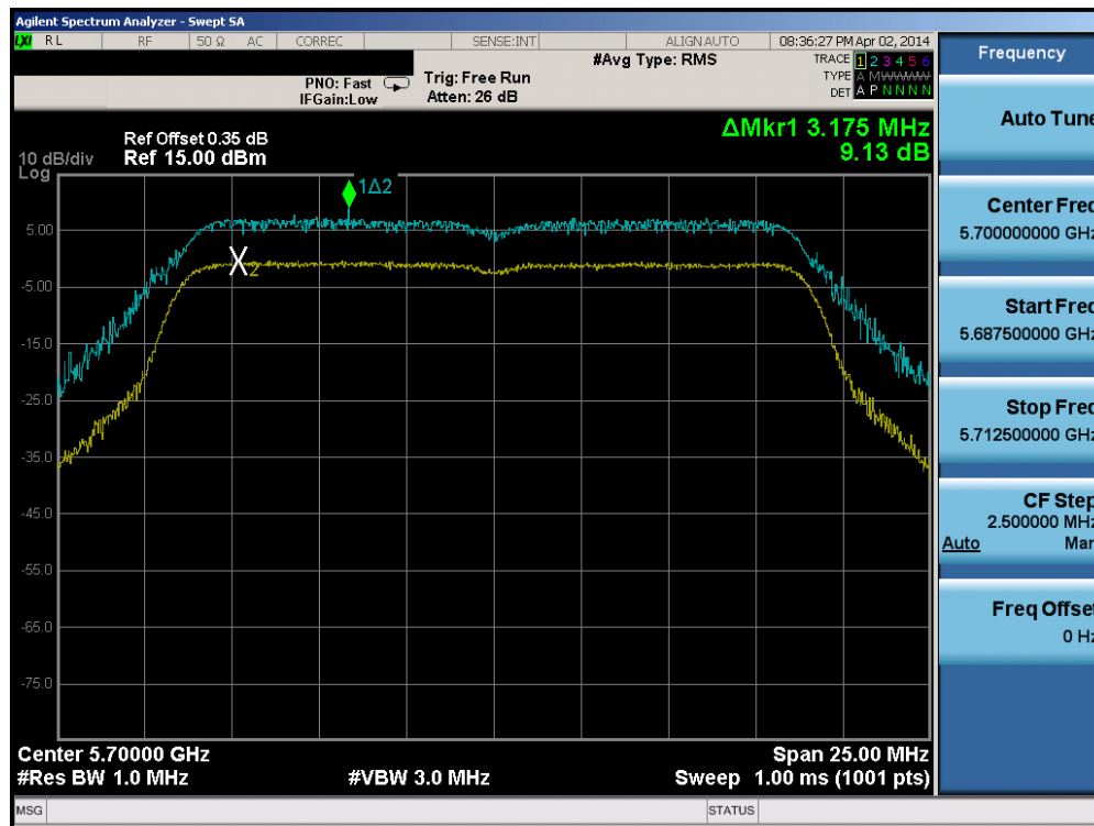
Plot 6-66. Peak Excursion Ratio Plot (20MHz BW 802.11n (UNII Band 2C) – Ch. 140)
