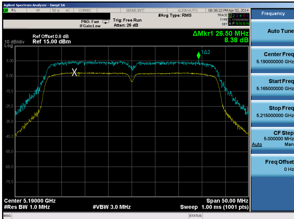
Plot 6-63. Peak Excursion Ratio Plot (40MHz BW 802.11n (UNII Band 1) – Ch. 38)
