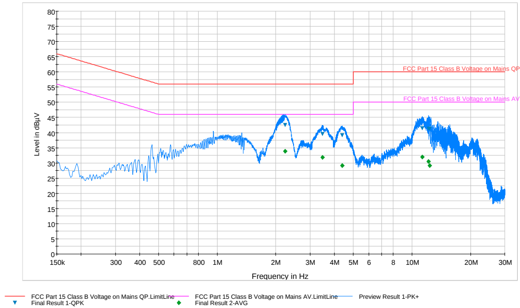
Plot 6-96. Line Conducted Plot with 802.11a UNII Band 2A (N)
