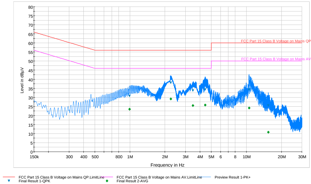
Plot 6-95. Line Conducted Plot with 802.11a UNII Band 2A (L1)
