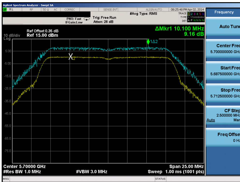
Plot 6-65. Peak Excursion Ratio Plot (802.11a (UNII Band 2C) – Ch. 140)
