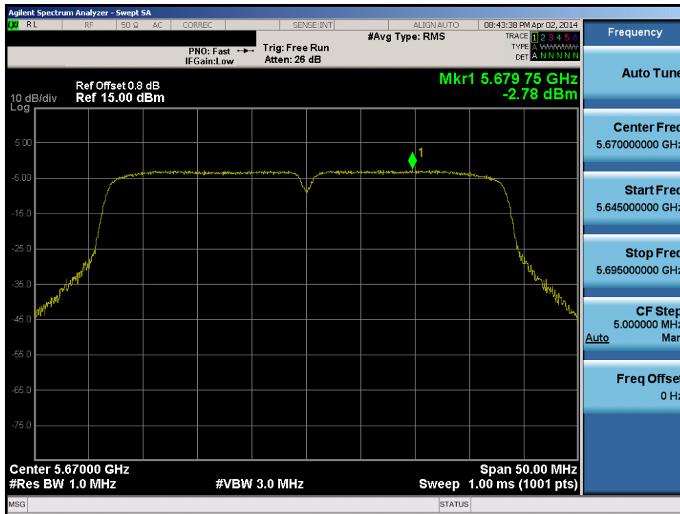
Plot 6-61. Peak Power Spectral Density Plot (40MHz BW 802.11n (UNII Band 2C) – Ch. 134)
