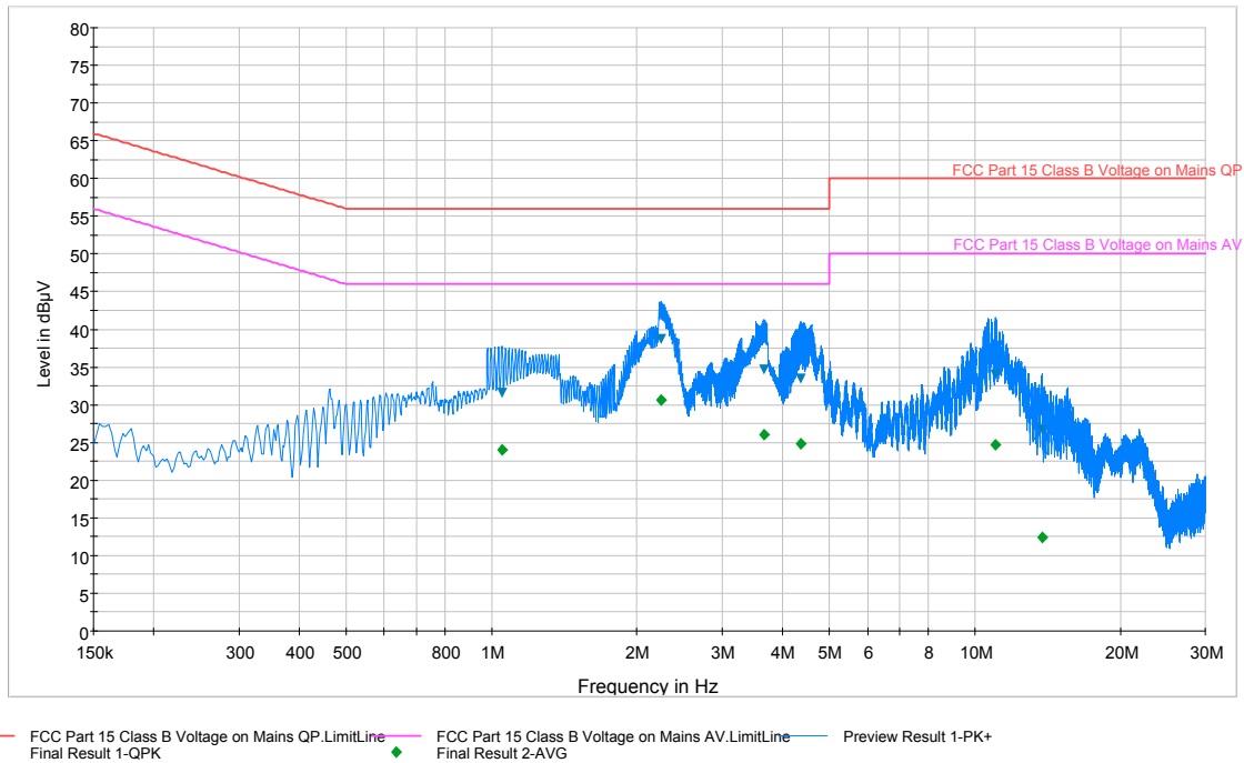
Plot 6-69. Line Conducted Plot with 802.11b (L1)
