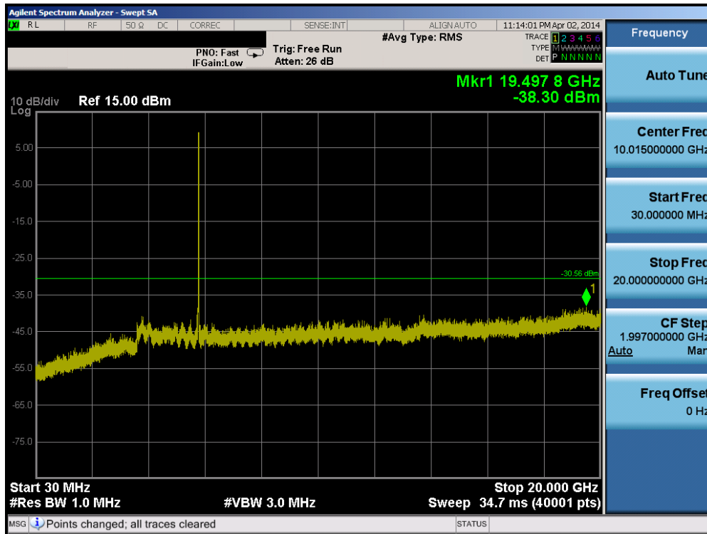
Plot 6-59. Conducted Spurious Plot (802.11a – Ch. 157)
