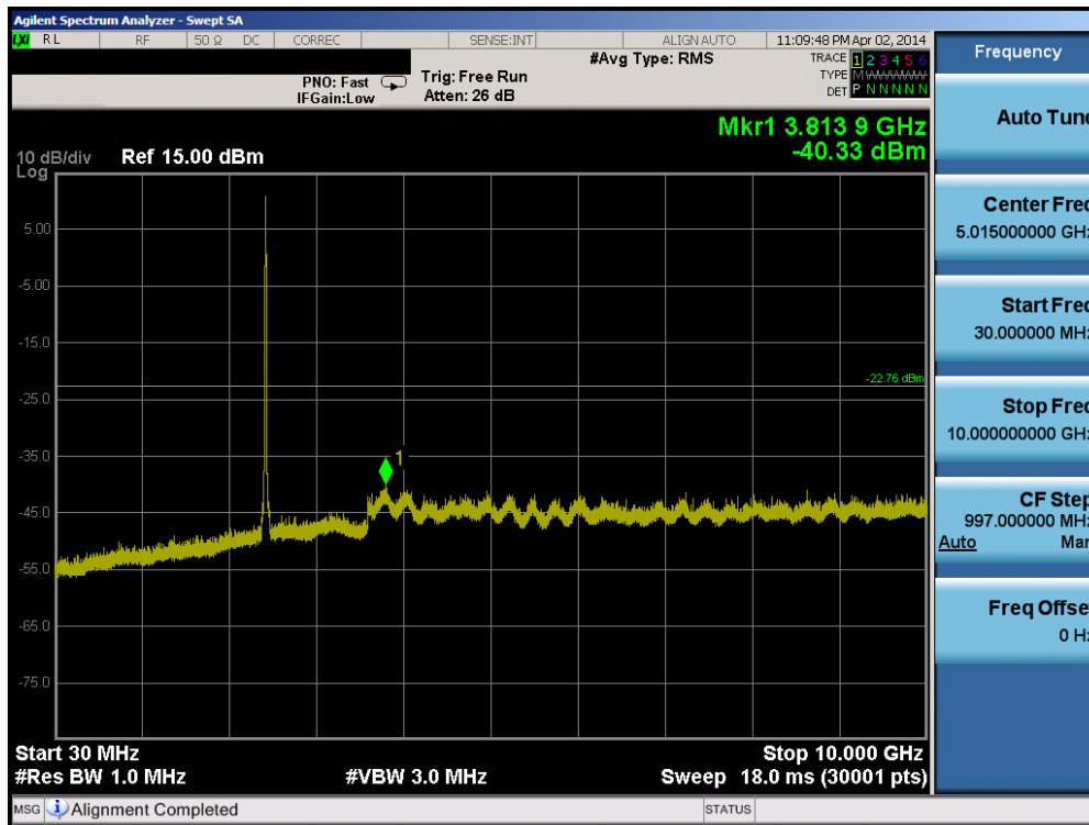
Plot 6-53. Conducted Spurious Plot (802.11b – Ch. 6)
