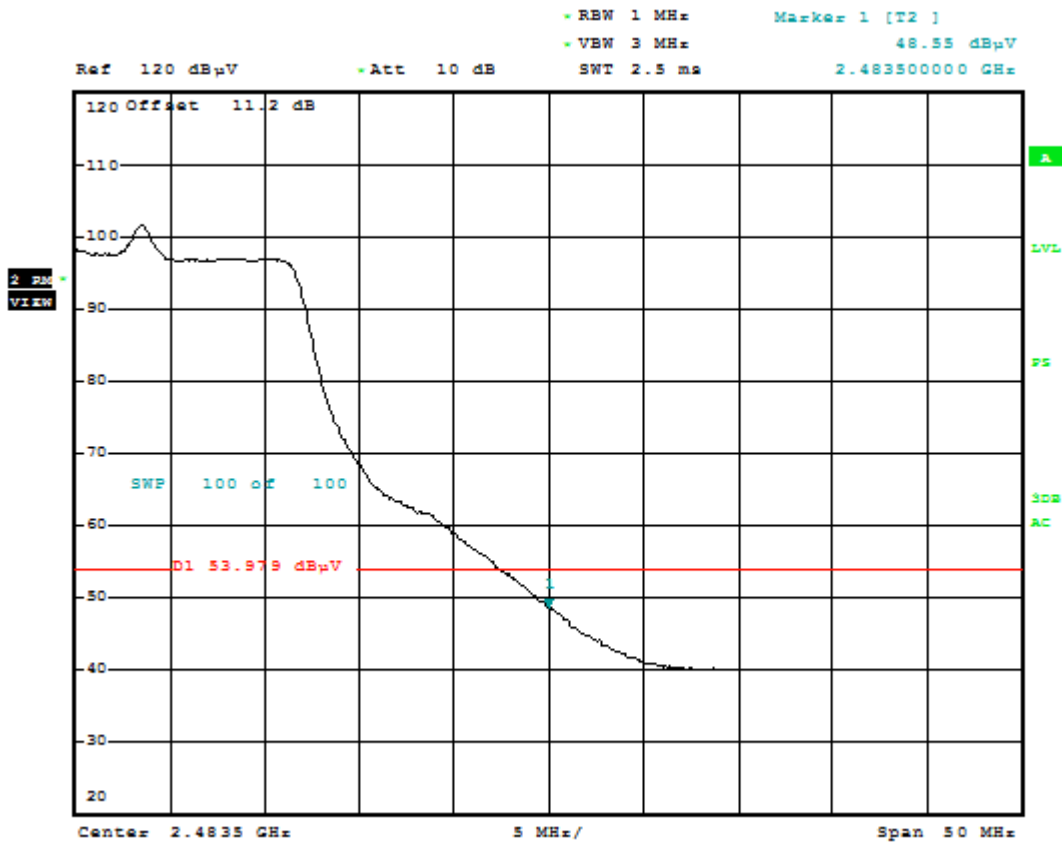
Plot 6-65. Radiated Restricted Upper Band Edge Measurement (Average)
