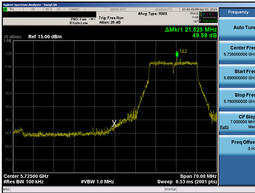
Plot 6-43. Band Edge Plot (802.11a – Ch. 149)
