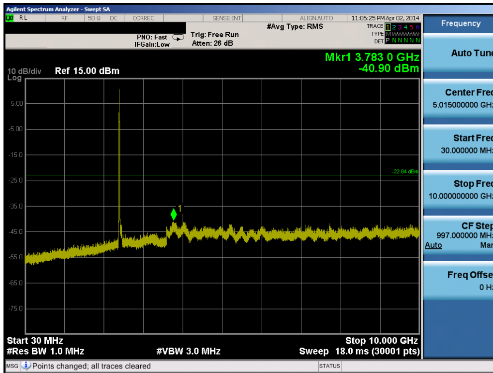
Plot 6-51. Conducted Spurious Plot (802.11b – Ch. 1)
