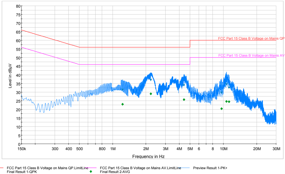
Plot 6-71. Line Conducted Plot with 802.11a (L1)
