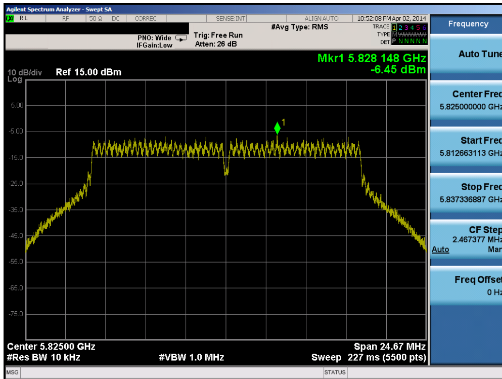
Plot 6-30. Power Spectral Density Plot (802.11a – Ch. 165)
