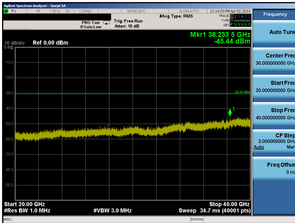
Plot 6-60. Conducted Spurious Plot (802.11a – Ch. 157)
