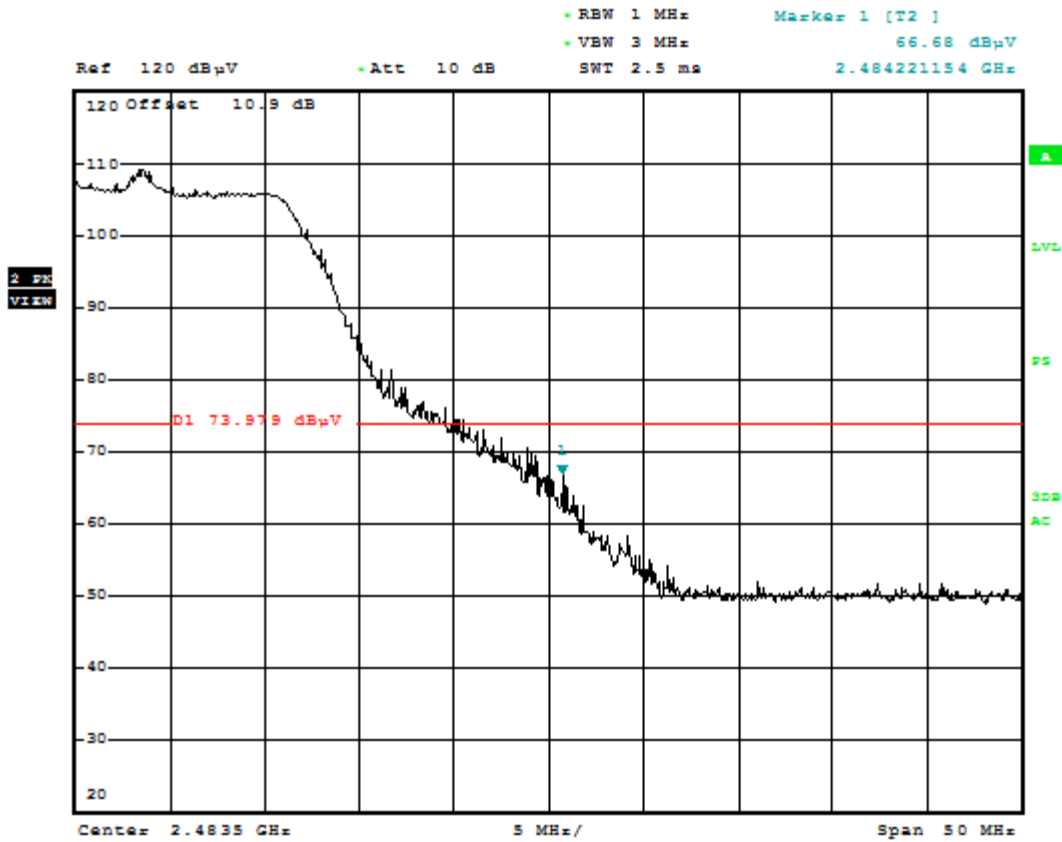
Plot 6-66. Radiated Restricted Upper Band Edge Measurement (Peak)
