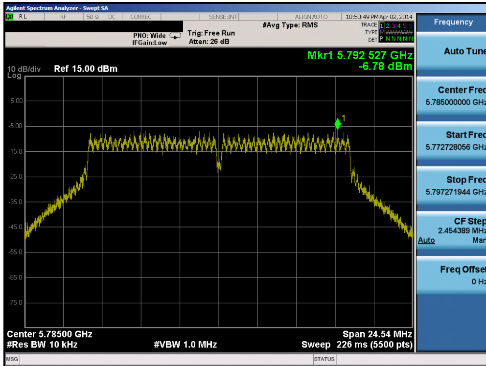
Plot 6-29. Power Spectral Density Plot (802.11a – Ch. 157)
