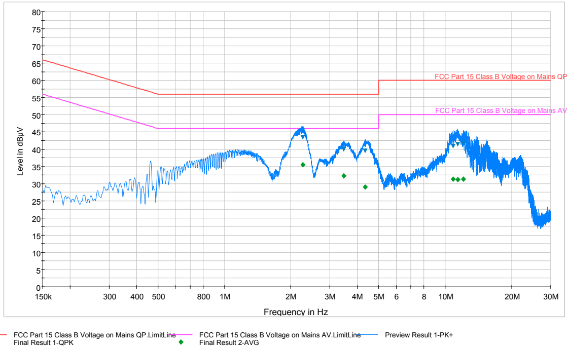
Plot 6-70. Line Conducted Plot with 802.11b (N)
