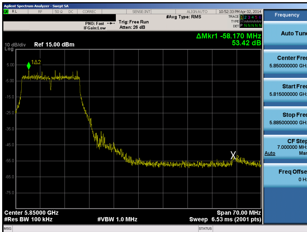
Plot 6-44. Band Edge Plot (802.11a – Ch. 165)
