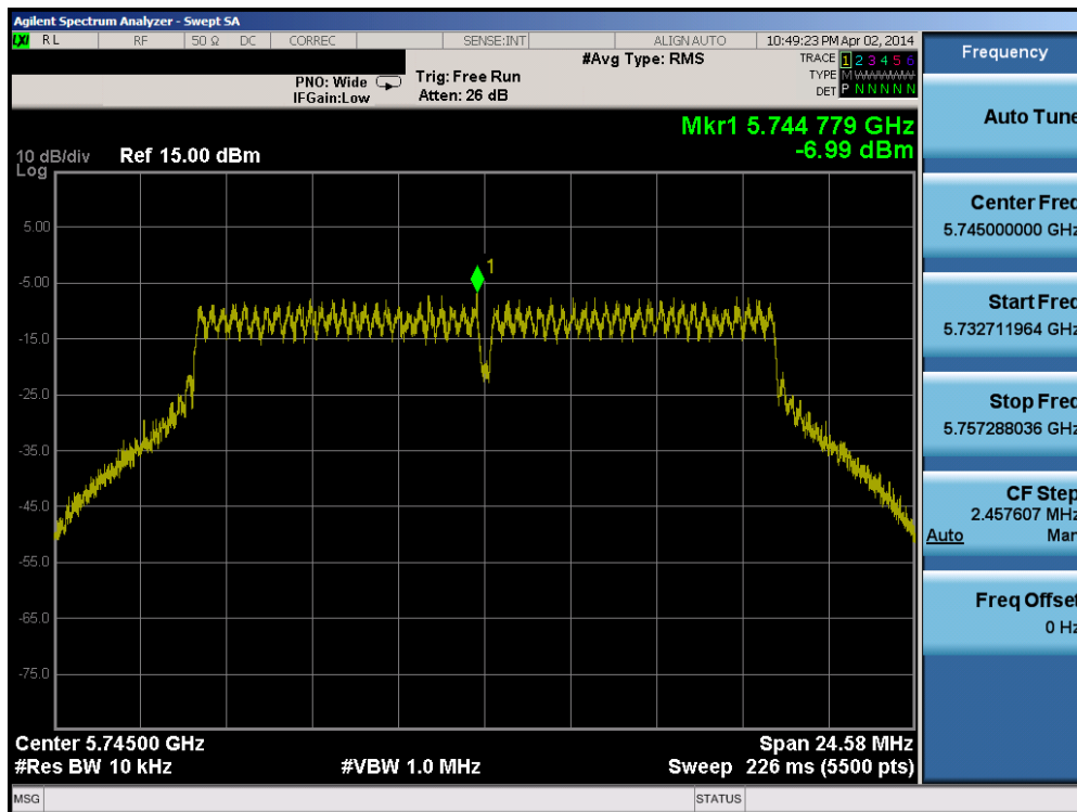
Plot 6-28. Power Spectral Density Plot (802.11a – Ch. 149)
