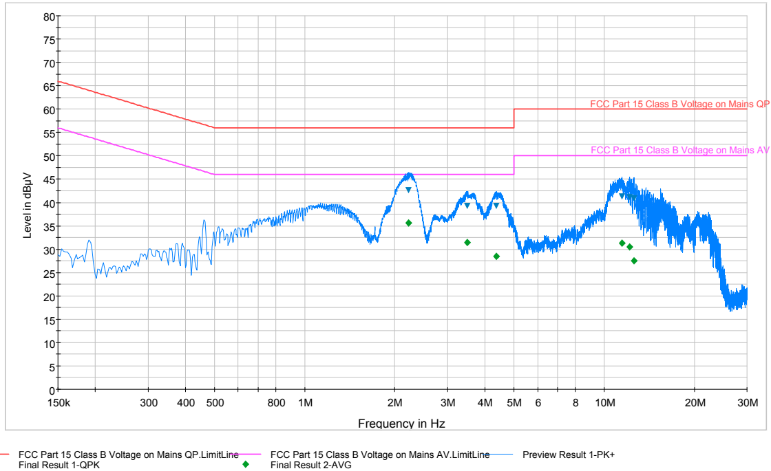
Plot 6-72. Line Conducted Plot with 802.11a (N)
