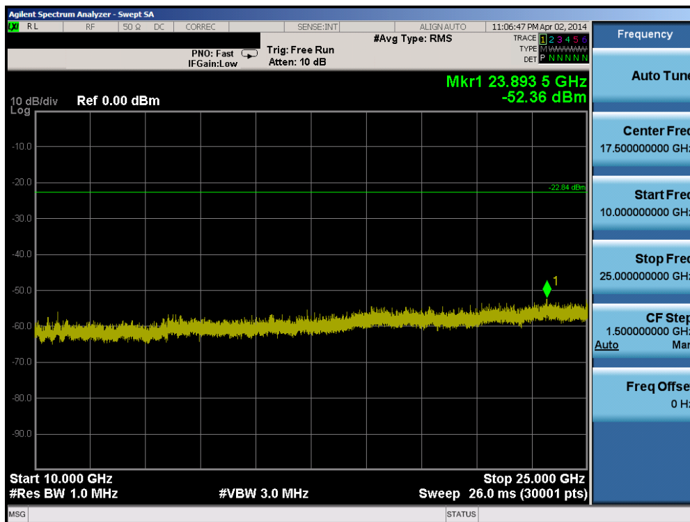
Plot 6-52. Conducted Spurious Plot (802.11b – Ch. 1)
