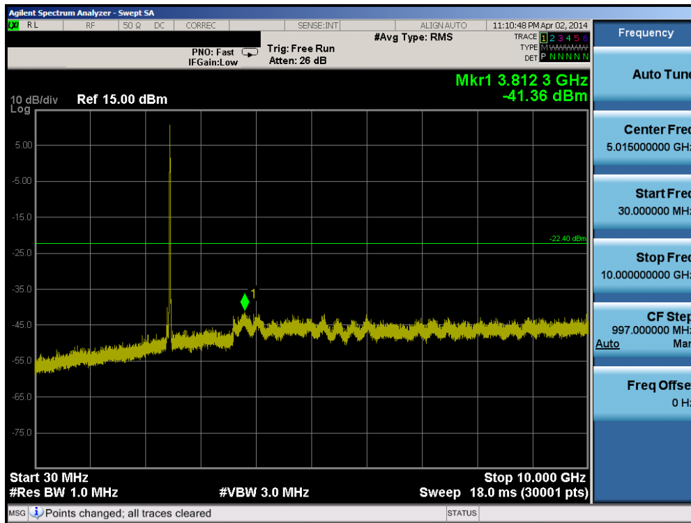
Plot 6-55. Conducted Spurious Plot (802.11b – Ch. 11)
