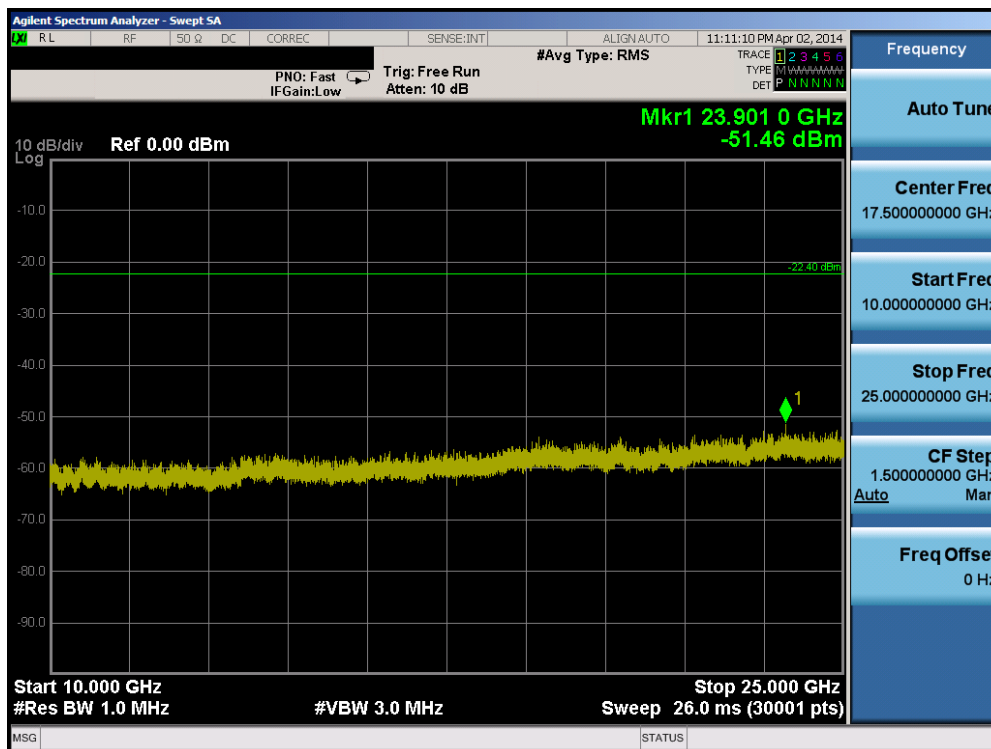
Plot 6-56. Conducted Spurious Plot (802.11b – Ch. 11)
