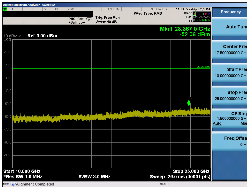
Plot 6-54. Conducted Spurious Plot (802.11b – Ch. 6)
