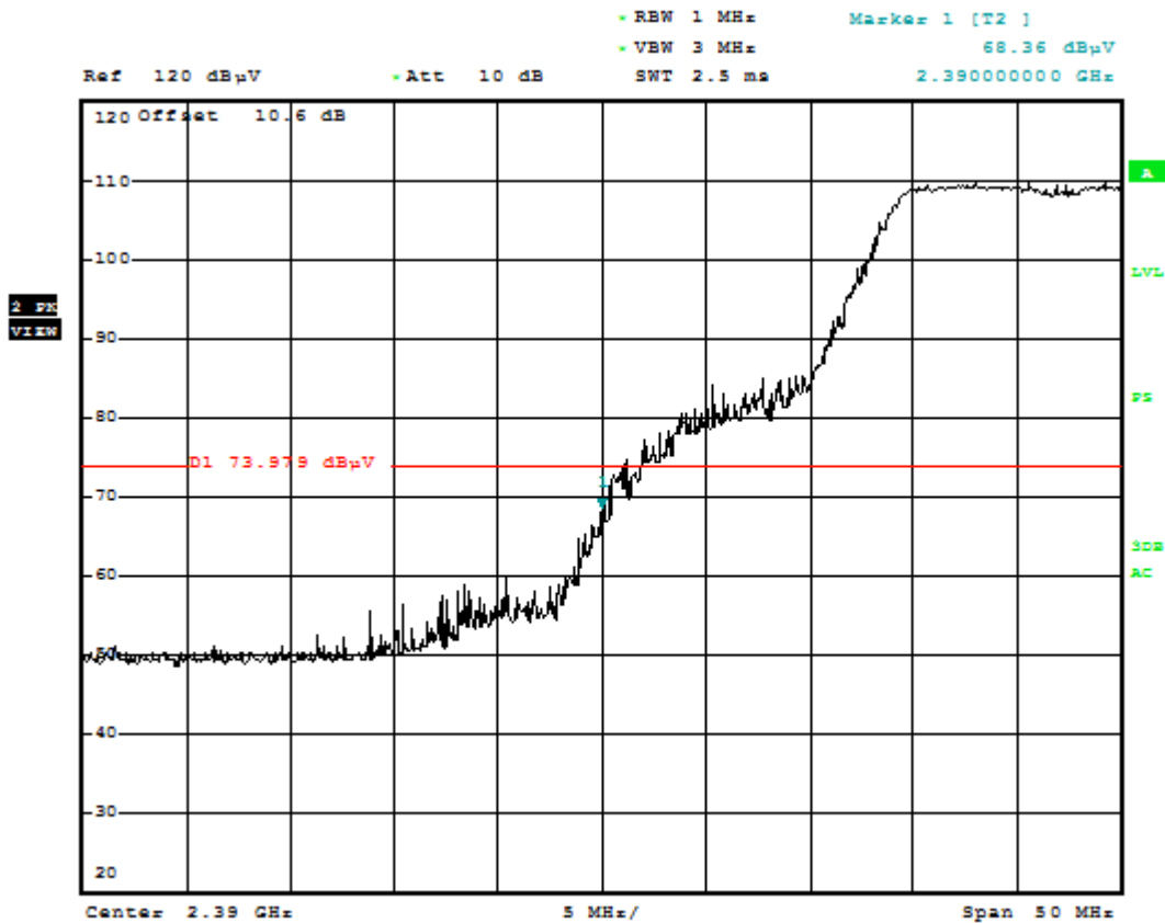
Plot 6-64. Radiated Restricted Lower Band Edge Measurement (Peak)
