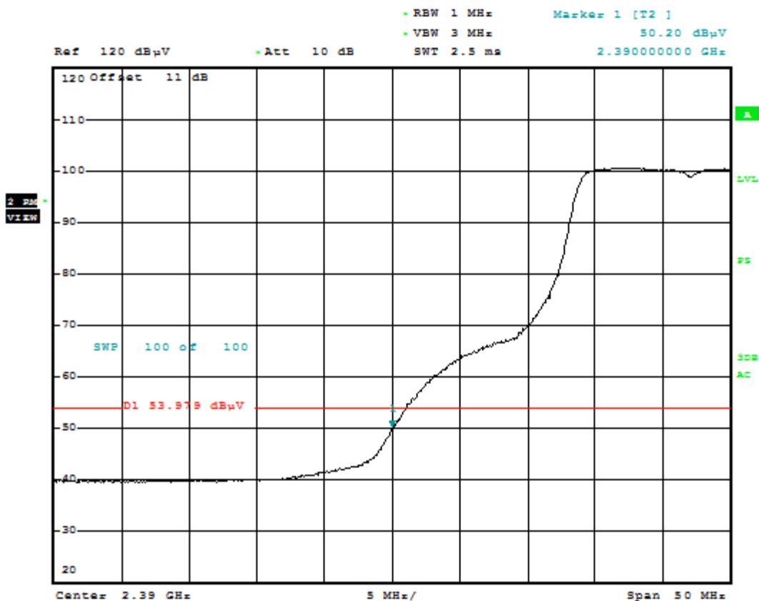
Plot 6-63. Radiated Restricted Lower Band Edge Measurement (Average)
