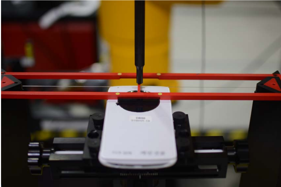
Figure 18-3 Ear Reference Point HAC Phantom Alignment, Wireless Charging Battery Cover (Cover Closed)
