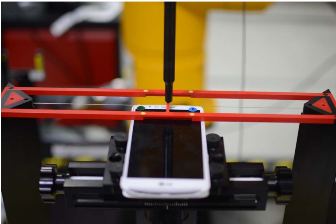
Figure 18-2 Ear Reference Point HAC Phantom Alignment, Wireless Charging Battery Cover (Cover Open)
