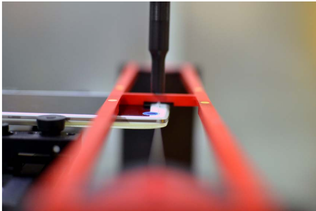
Figure 18-4 HAC Phantom Plane Alignment
