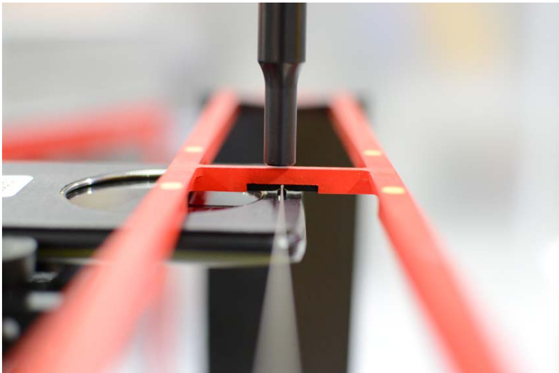
Figure 18-6 HAC Phantom Plane Alignment, Wireless Charging Cover (Cover Closed)
