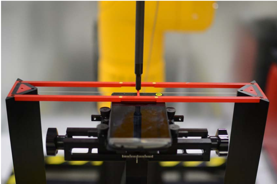
Figure 18-2 Ear Reference Point HAC Phantom Alignment, Wireless Charging Cover (Cover Open)
