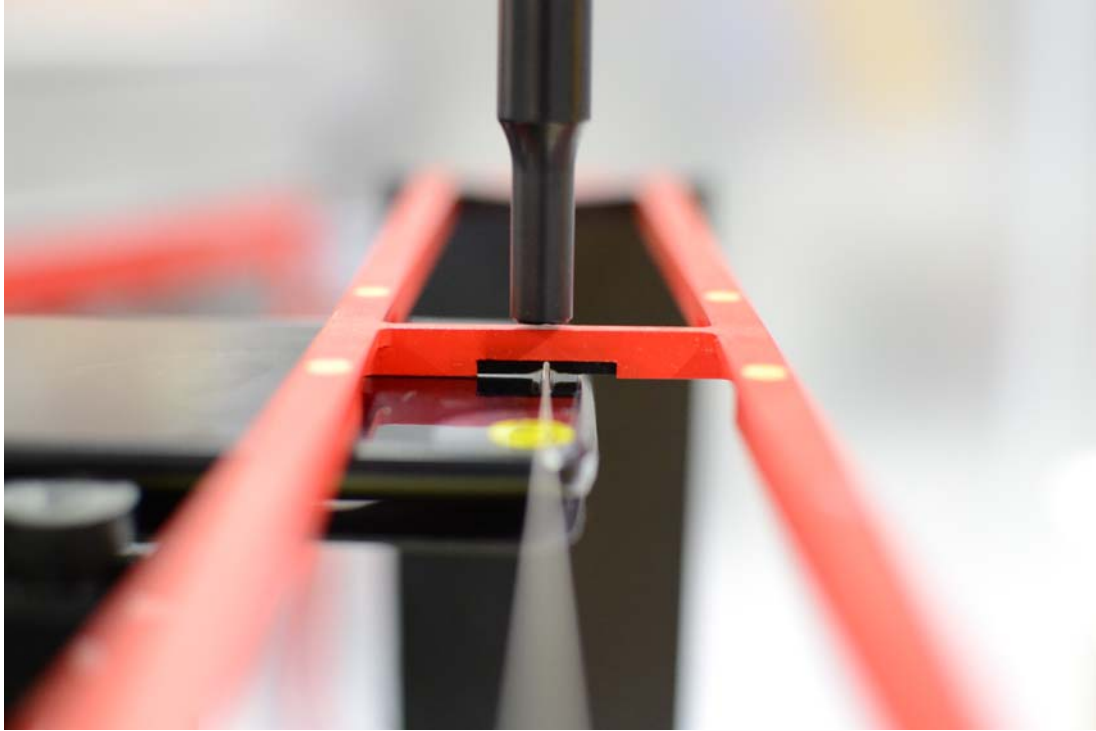
Figure 18-5 HAC Phantom Plane Alignment, Wireless Charging Cover (Cover Open)
