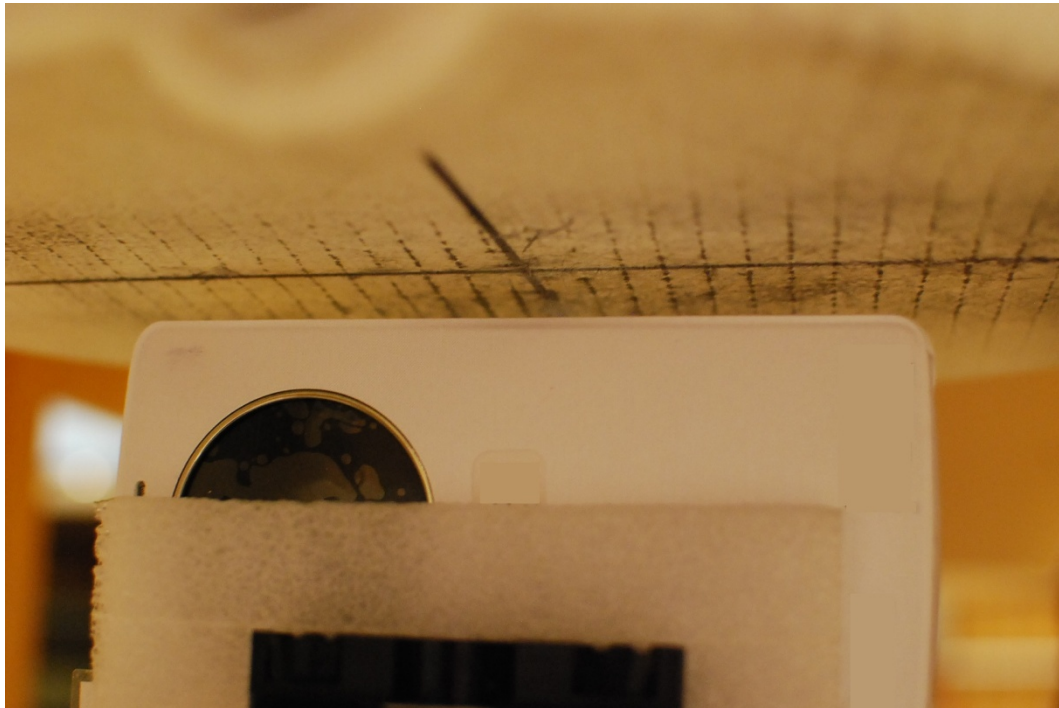
SAR Test Setup Photo 18 - Right Edge at 10 mm with WCC closed
