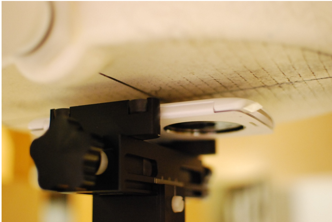
SAR Test Setup Photo 12 - Back at 10 mm with WCC closed
