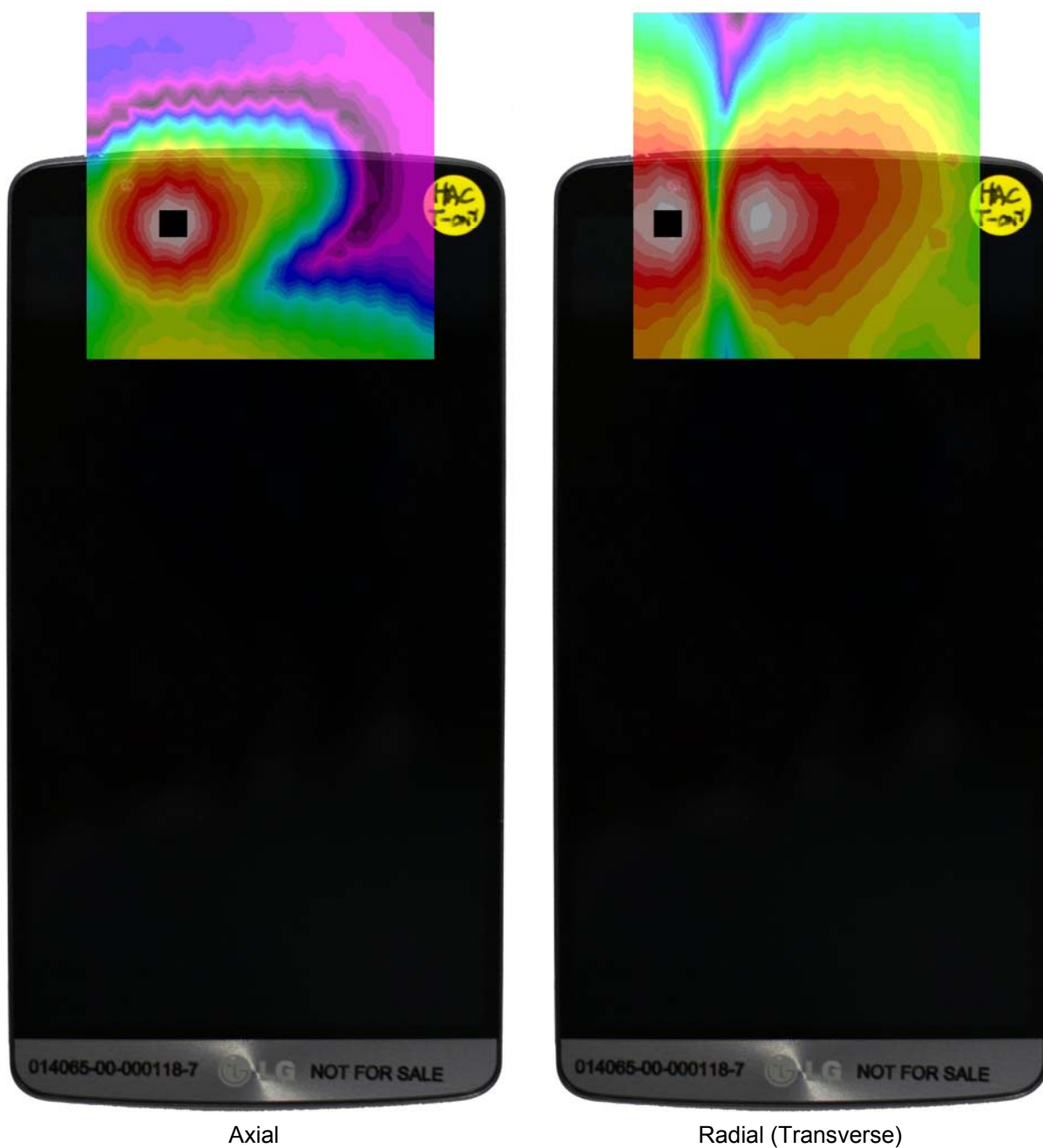
Figure 13-7 T-Coil Scan Overlay Magnetic Field Distributions
