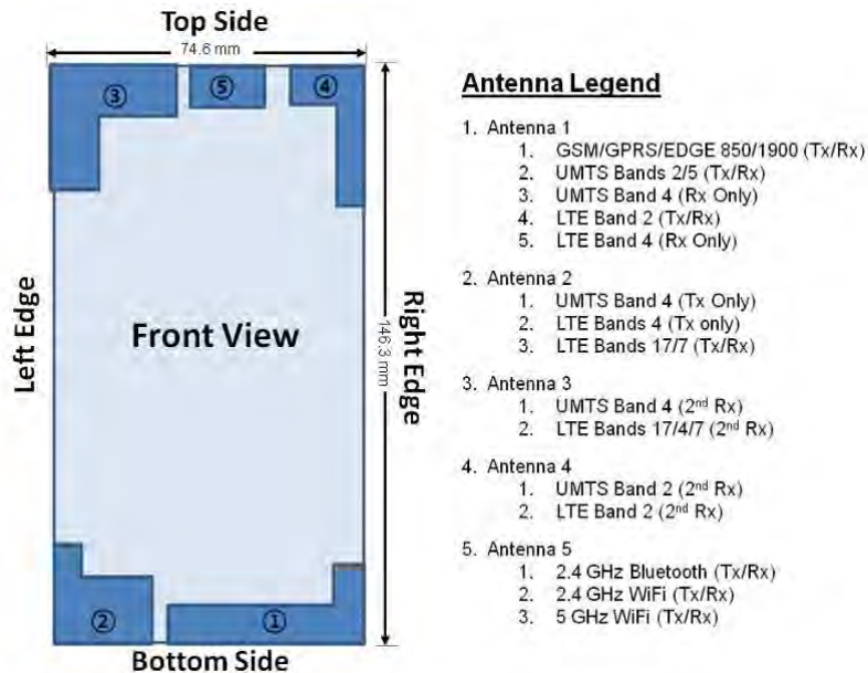
Figure 1-1 DUT Antenna Locations
