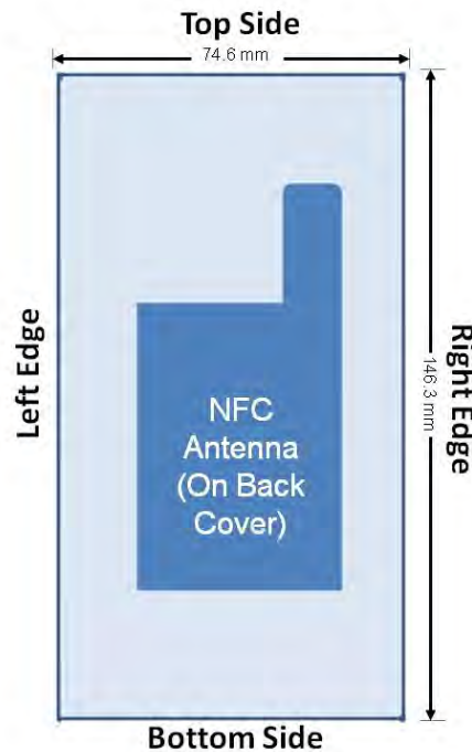
Figure 1-2 NFC Antenna Locations
