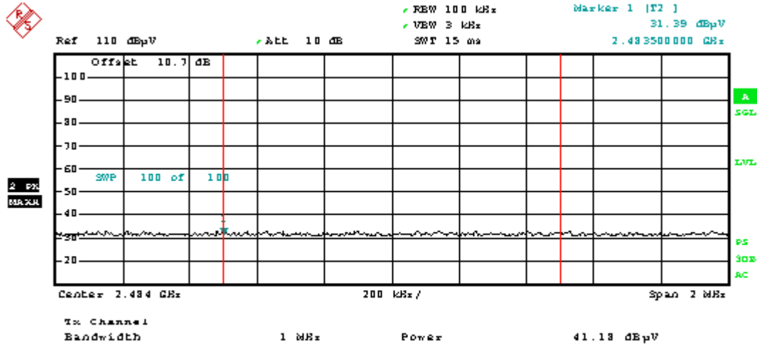
Plot 6-3. Radiated Restricted Upper Band Edge Measurement with WCC (Average)
