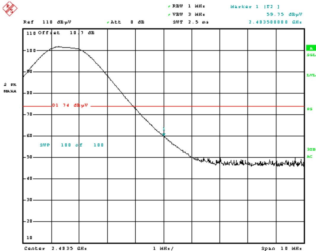
Plot 6-2. Radiated Restricted Upper Band Edge Measurement (Peak)
