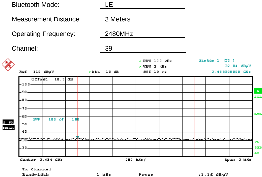
Plot 6-1. Radiated Restricted Upper Band Edge Measurement (Average)
