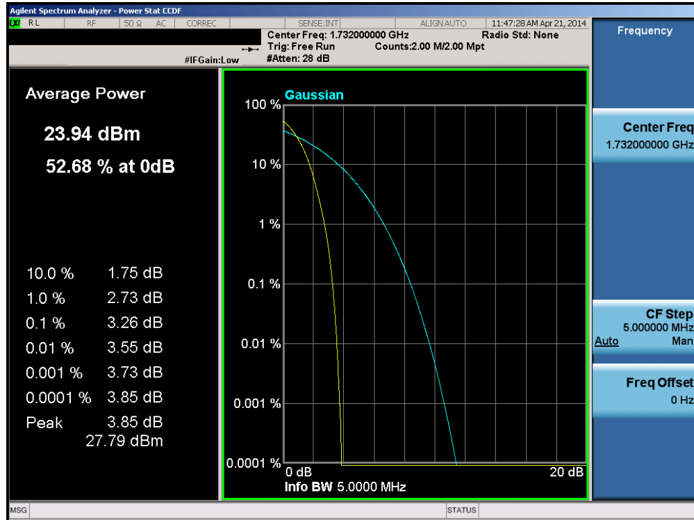
Plot 6-57. Peak-Average Ratio Plot (AWS WCDMA Mode – Ch. 1412)
