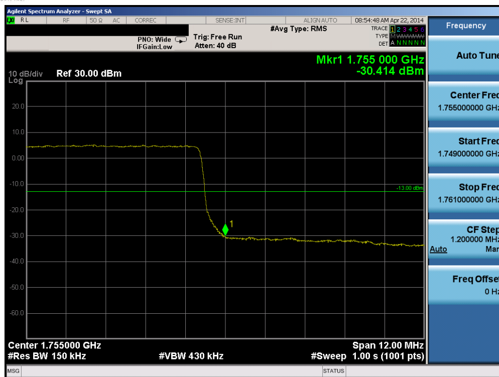
Plot 6-113. Upper Band Edge Plot (Band 4 – 15.0MHz QPSK – RB Size 75)
