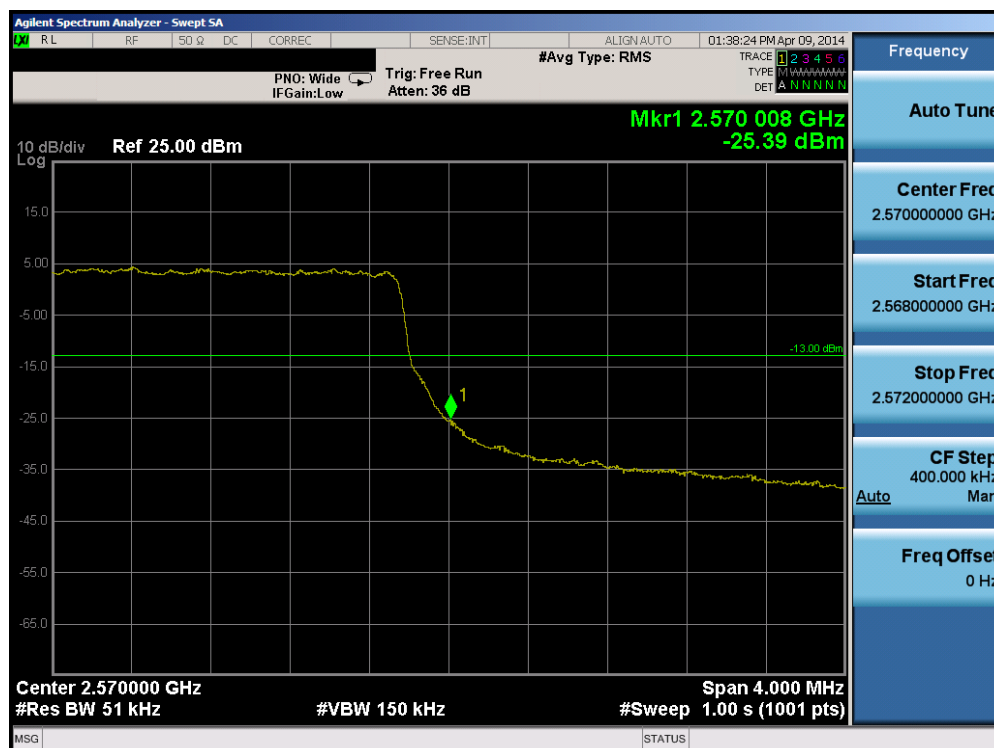
Plot 6-136. Upper Band Edge Plot (Band 7 – 5.0MHz QPSK – RB Size 25)
